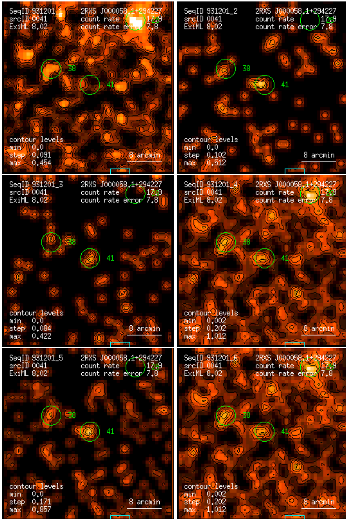
Figure 41: RASS 931201: detection 0041: band rate images, Gaussian filter: (1) PSPC channels 11 – 41, (2) 52 – 90, (3) 91 – 201, (4) 11 – 235, (5) 52 – 201, (6) 11 – 201. Broad band rates in counts/ks. Band rate contour levels in counts/ks/arcmin 2 .
