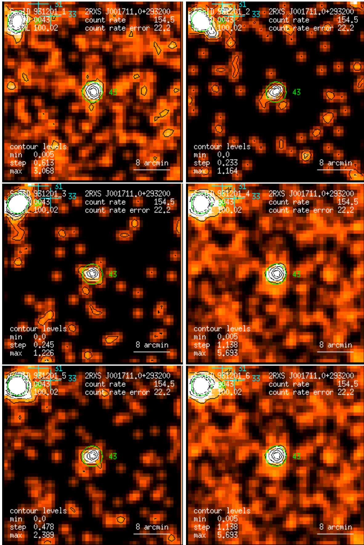
Figure 43: RASS 931201: detection 0043: band rate images, Gaussian filter: (1) PSPC channels 11 – 41, (2) 52 – 90, (3) 91 – 201, (4) 11 – 235, (5) 52 – 201, (6) 11 – 201. Broad band rates in counts/ks. Band rate contour levels in counts/ks/arcmin 2 .
