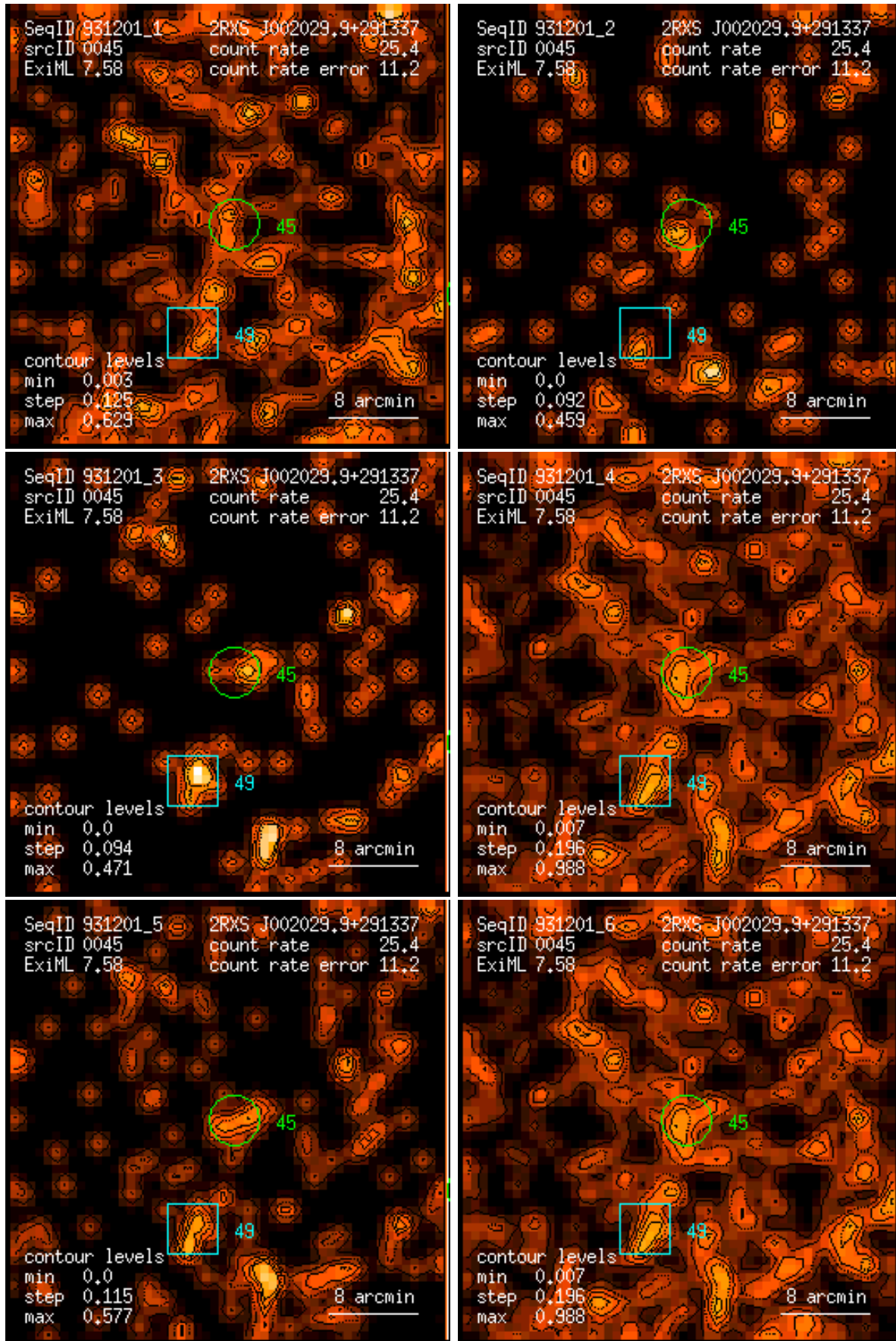
Figure 45: RASS 931201: detection 0045: band rate images, Gaussian filter: (1) PSPC channels 11 – 41, (2) 52 – 90, (3) 91 – 201, (4) 11 – 235, (5) 52 – 201, (6) 11 – 201. Broad band rates in counts/ks. Band rate contour levels in counts/ks/arcmin 2 .
