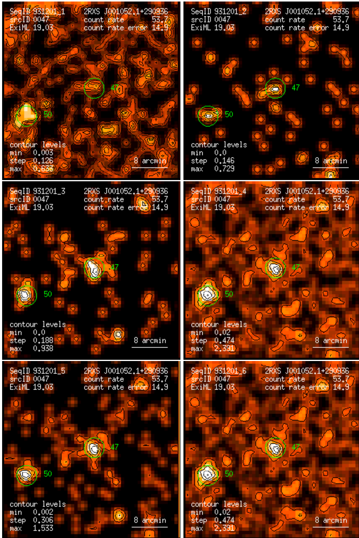
Figure 47: RASS 931201: detection 0047: band rate images, Gaussian filter: (1) PSPC channels 11 – 41, (2) 52 – 90, (3) 91 – 201, (4) 11 – 235, (5) 52 – 201, (6) 11 – 201. Broad band rates in counts/ks. Band rate contour levels in counts/ks/arcmin 2 .
