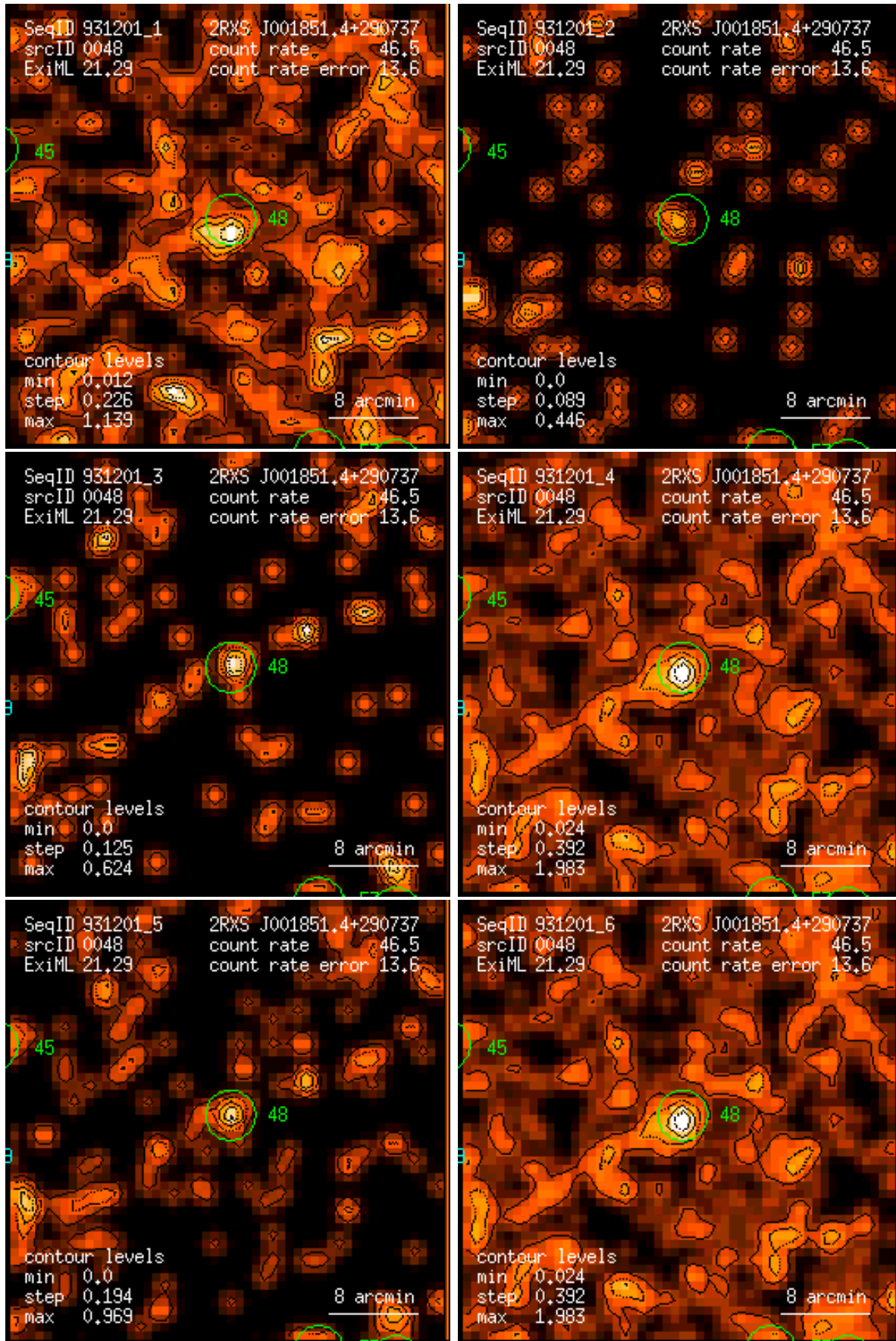
Figure 48: RASS 931201: detection 0048: band rate images, Gaussian filter: (1) PSPC channels 11 – 41, (2) 52 – 90, (3) 91 – 201, (4) 11 – 235, (5) 52 – 201, (6) 11 – 201. Broad band rates in counts/ks. Band rate contour levels in counts/ks/arcmin 2 .
