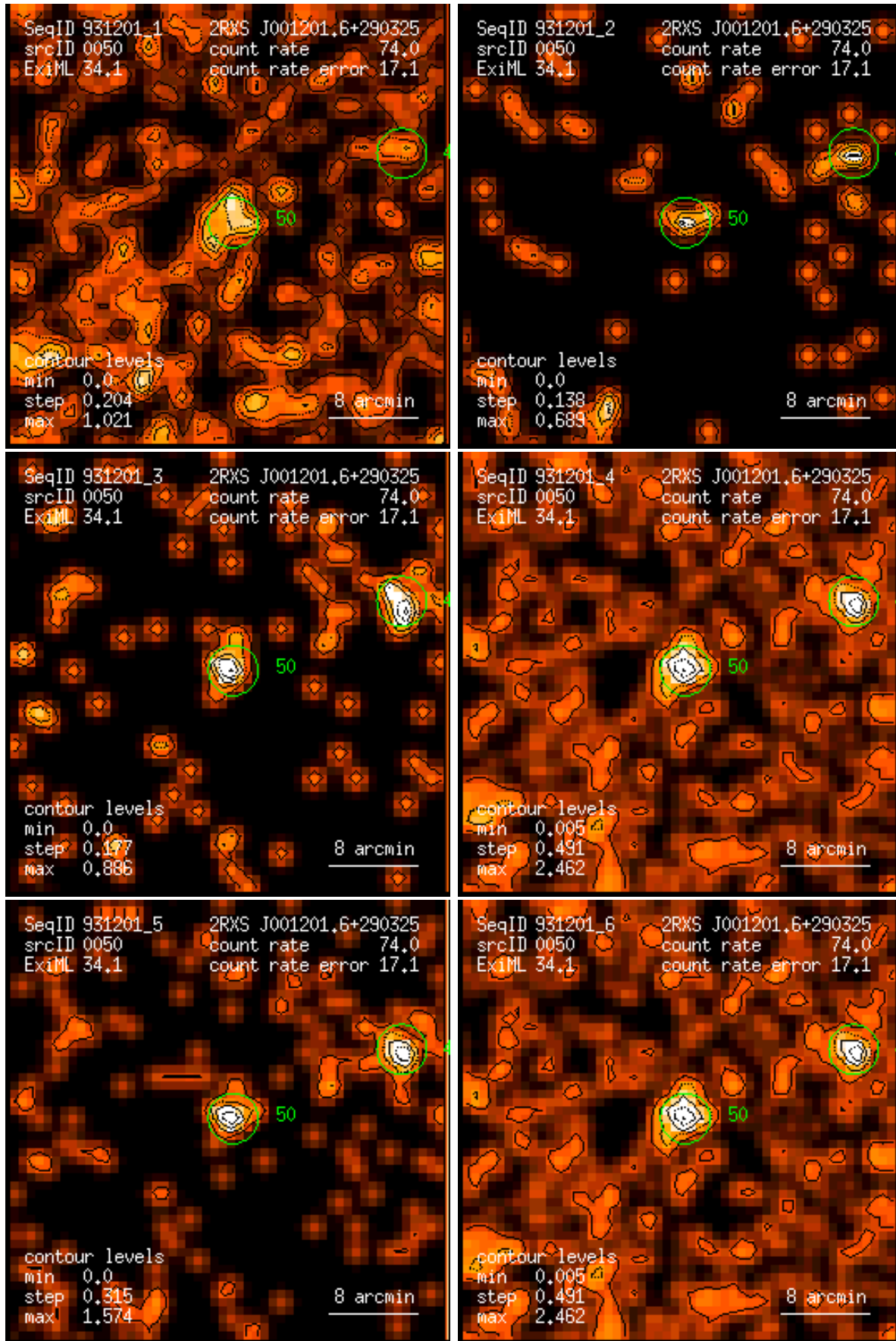
Figure 50: RASS 931201: detection 0050: band rate images, Gaussian filter: (1) PSPC channels 11 – 41, (2) 52 – 90, (3) 91 – 201, (4) 11 – 235, (5) 52 – 201, (6) 11 – 201. Broad band rates in counts/ks. Band rate contour levels in counts/ks/arcmin 2 .
