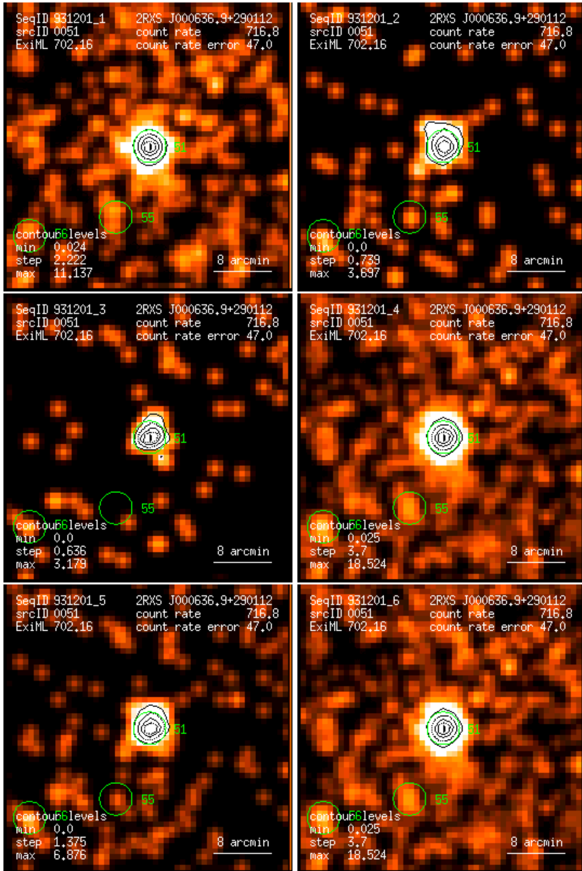
Figure 51: RASS 931201: detection 0051: band rate images, Gaussian filter: (1) PSPC channels 11 – 41, (2) 52 – 90, (3) 91 – 201, (4) 11 – 235, (5) 52 – 201, (6) 11 – 201. Broad band rates in counts/ks. Band rate contour levels in counts/ks/arcmin 2 .
