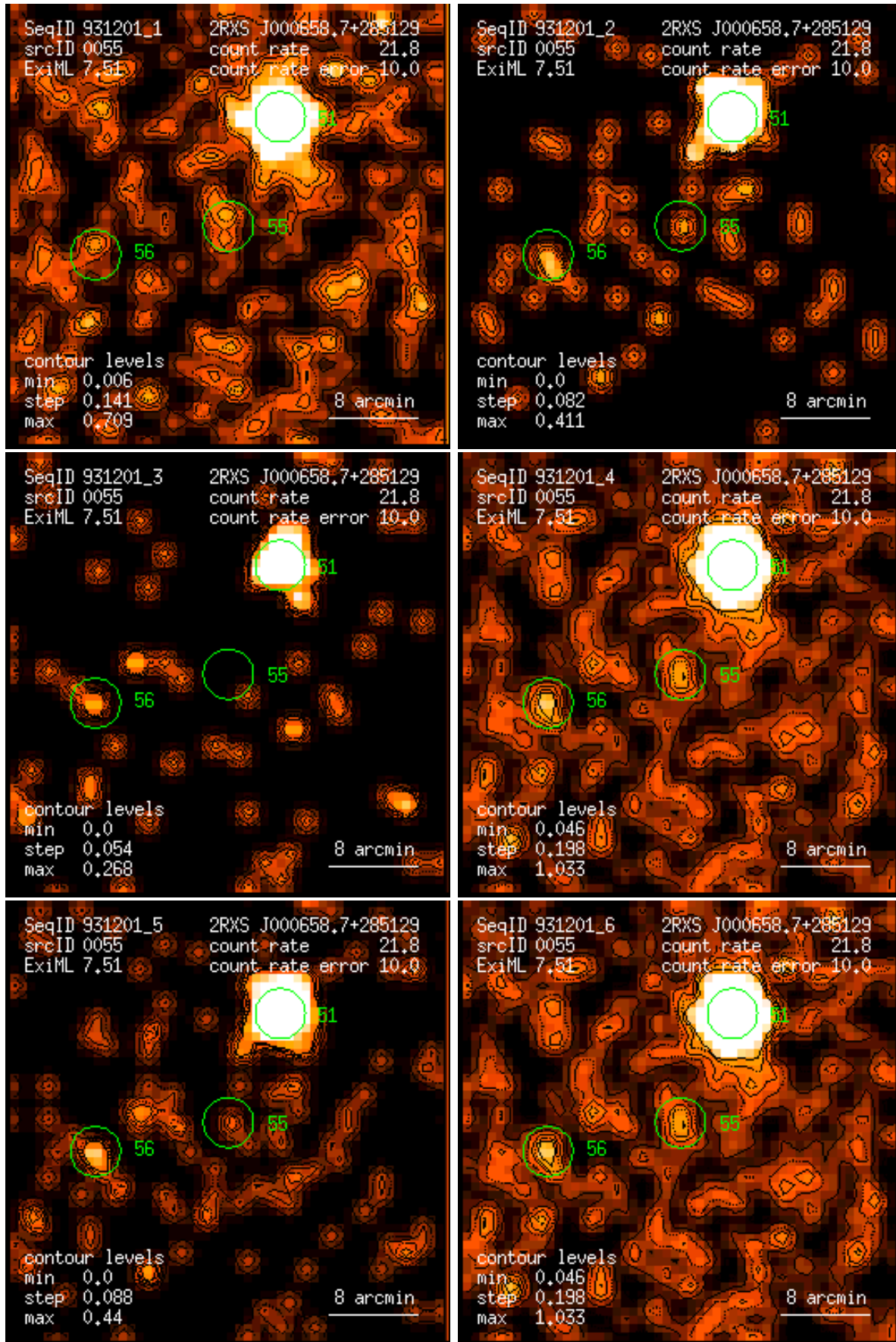
Figure 55: RASS 931201: detection 0055: band rate images, Gaussian filter: (1) PSPC channels 11 – 41, (2) 52 – 90, (3) 91 – 201, (4) 11 – 235, (5) 52 – 201, (6) 11 – 201. Broad band rates in counts/ks. Band rate contour levels in counts/ks/arcmin 2 .
