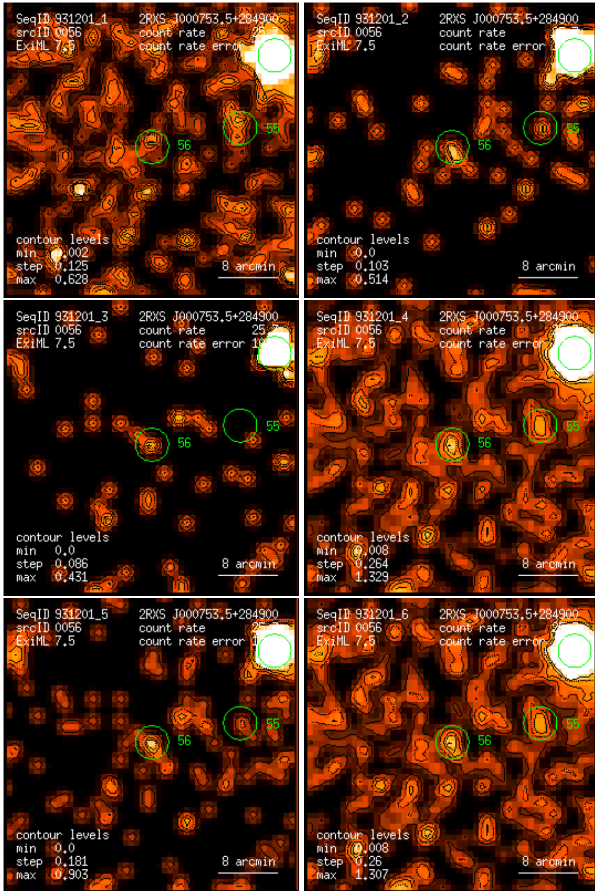
Figure 56: RASS 931201: detection 0056: band rate images, Gaussian filter: (1) PSPC channels 11 – 41, (2) 52 – 90, (3) 91 – 201, (4) 11 – 235, (5) 52 – 201, (6) 11 – 201. Broad band rates in counts/ks. Band rate contour levels in counts/ks/arcmin 2 .
