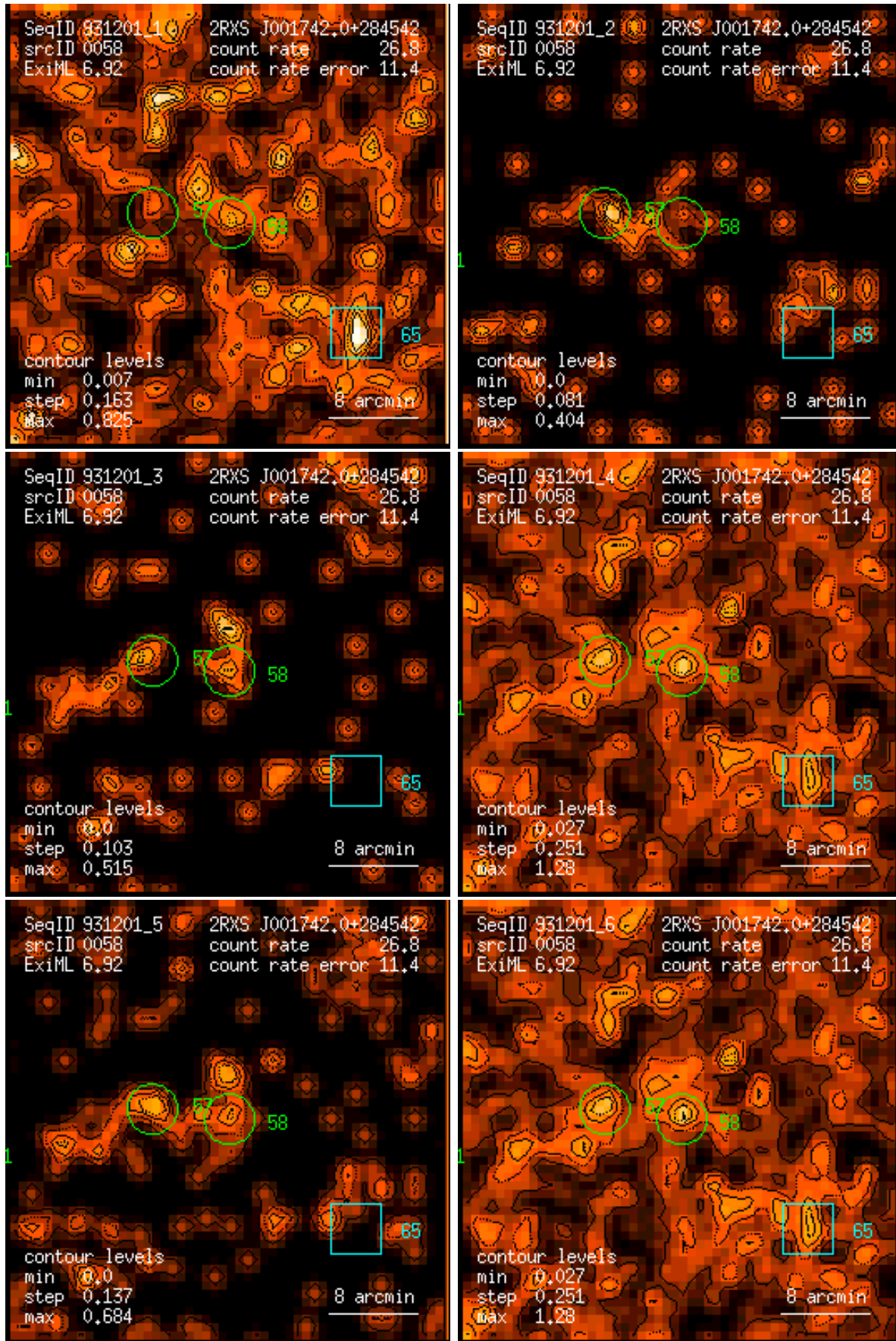
Figure 58: RASS 931201: detection 0058: band rate images, Gaussian filter: (1) PSPC channels 11 – 41, (2) 52 – 90, (3) 91 – 201, (4) 11 – 235, (5) 52 – 201, (6) 11 – 201. Broad band rates in counts/ks. Band rate contour levels in counts/ks/arcmin 2 .
