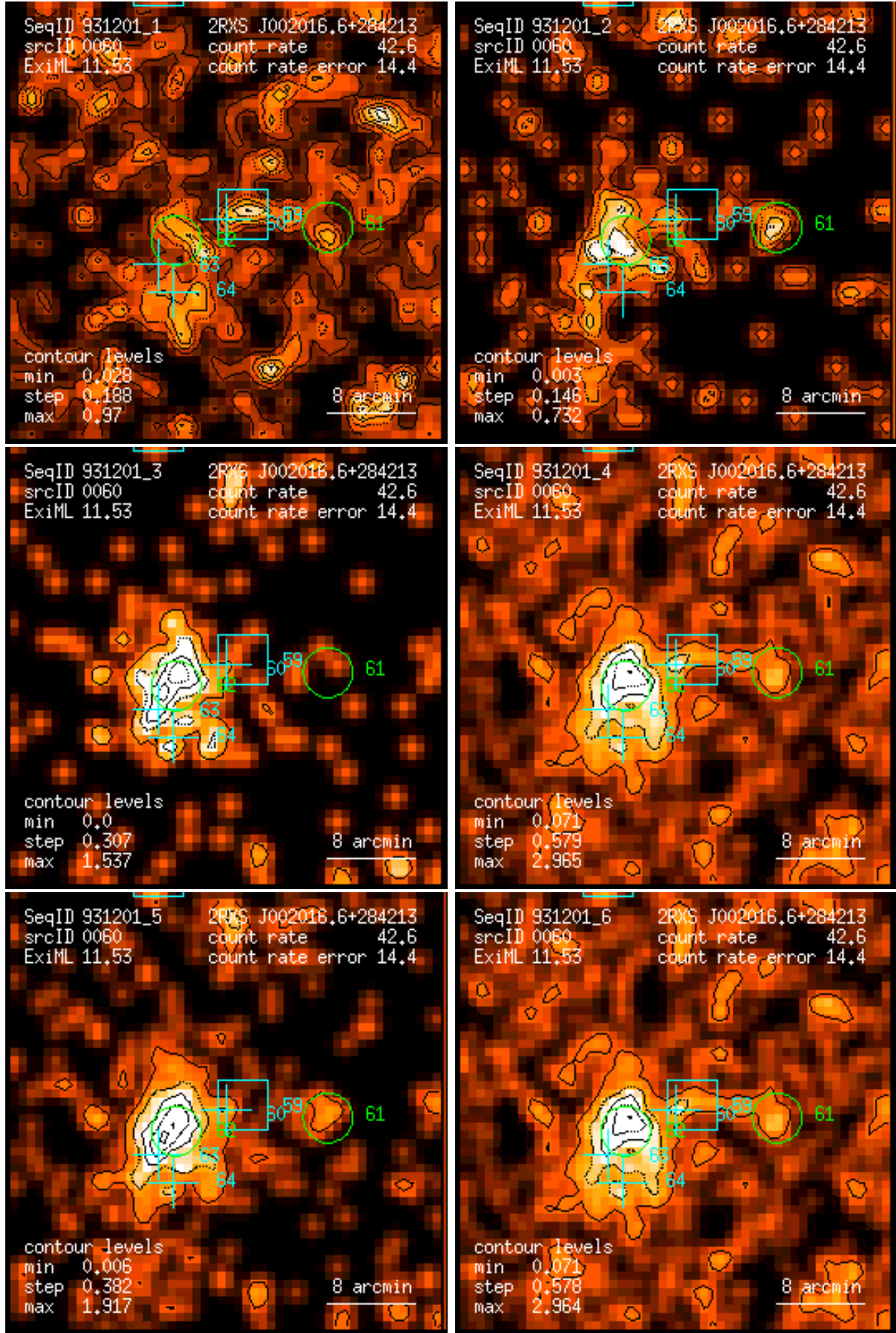
Figure 60: RASS 931201: detection 0060: band rate images, Gaussian filter: (1) PSPC channels 11 – 41, (2) 52 – 90, (3) 91 – 201, (4) 11 – 235, (5) 52 – 201, (6) 11 – 201. Broad band rates in counts/ks. Band rate contour levels in counts/ks/arcmin 2 .
