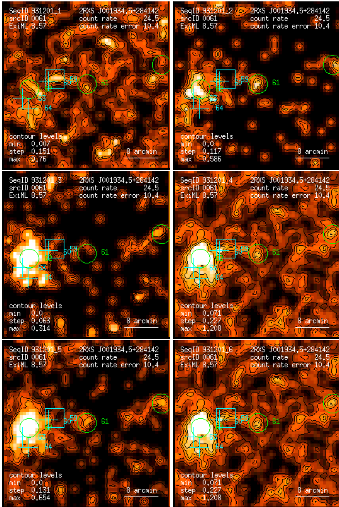
Figure 61: RASS 931201: detection 0061: band rate images, Gaussian filter: (1) PSPC channels 11 – 41, (2) 52 – 90, (3) 91 – 201, (4) 11 – 235, (5) 52 – 201, (6) 11 – 201. Broad band rates in counts/ks. Band rate contour levels in counts/ks/arcmin 2 .
