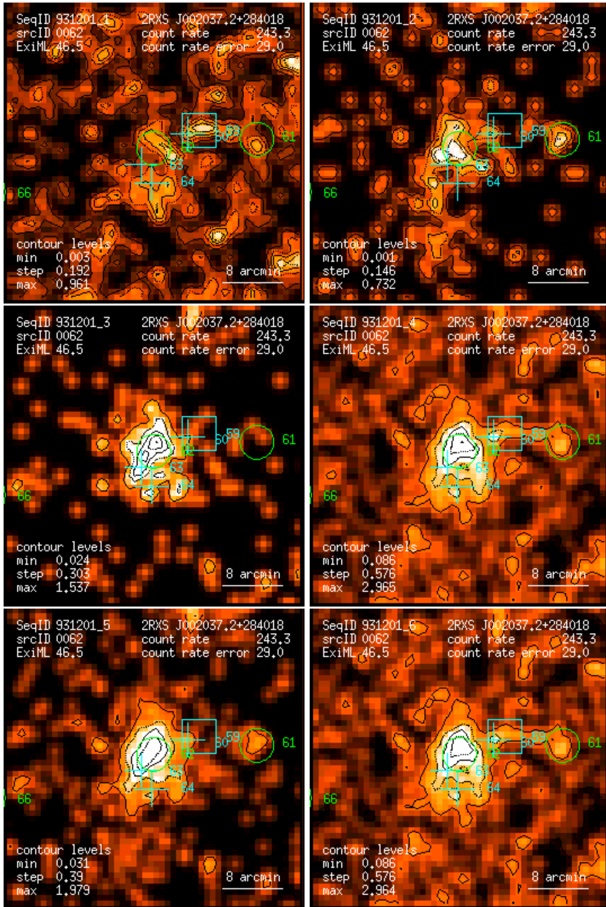
Figure 62: RASS 931201: detection 0062: band rate images, Gaussian filter: (1) PSPC channels 11 – 41, (2) 52 – 90, (3) 91 – 201, (4) 11 – 235, (5) 52 – 201, (6) 11 – 201. Broad band rates in counts/ks. Band rate contour levels in counts/ks/arcmin 2 .
