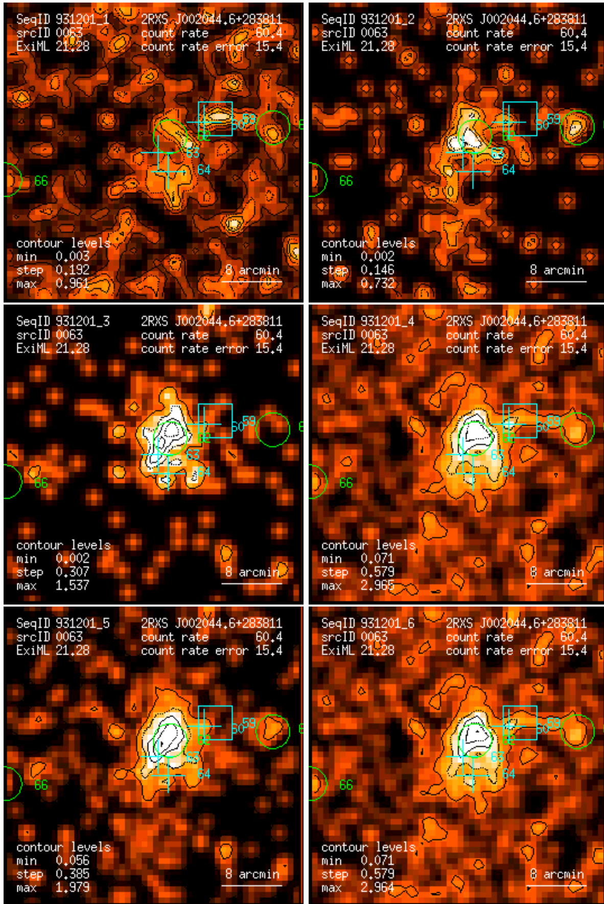
Figure 63: RASS 931201: detection 0063: band rate images, Gaussian filter: (1) PSPC channels 11 – 41, (2) 52 – 90, (3) 91 – 201, (4) 11 – 235, (5) 52 – 201, (6) 11 – 201. Broad band rates in counts/ks. Band rate contour levels in counts/ks/arcmin 2 .
