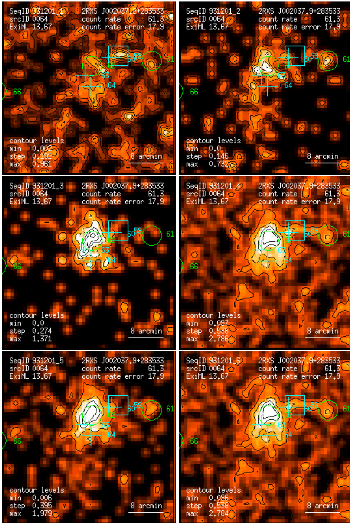
Figure 64: RASS 931201: detection 0064: band rate images, Gaussian filter: (1) PSPC channels 11 – 41, (2) 52 – 90, (3) 91 – 201, (4) 11 – 235, (5) 52 – 201, (6) 11 – 201. Broad band rates in counts/ks. Band rate contour levels in counts/ks/arcmin 2 .
