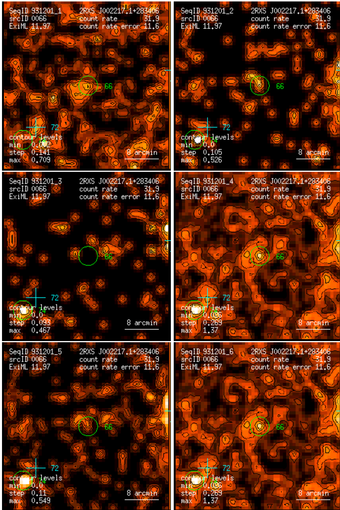
Figure 66: RASS 931201: detection 0066: band rate images, Gaussian filter: (1) PSPC channels 11 – 41, (2) 52 – 90, (3) 91 – 201, (4) 11 – 235, (5) 52 – 201, (6) 11 – 201. Broad band rates in counts/ks. Band rate contour levels in counts/ks/arcmin 2 .
