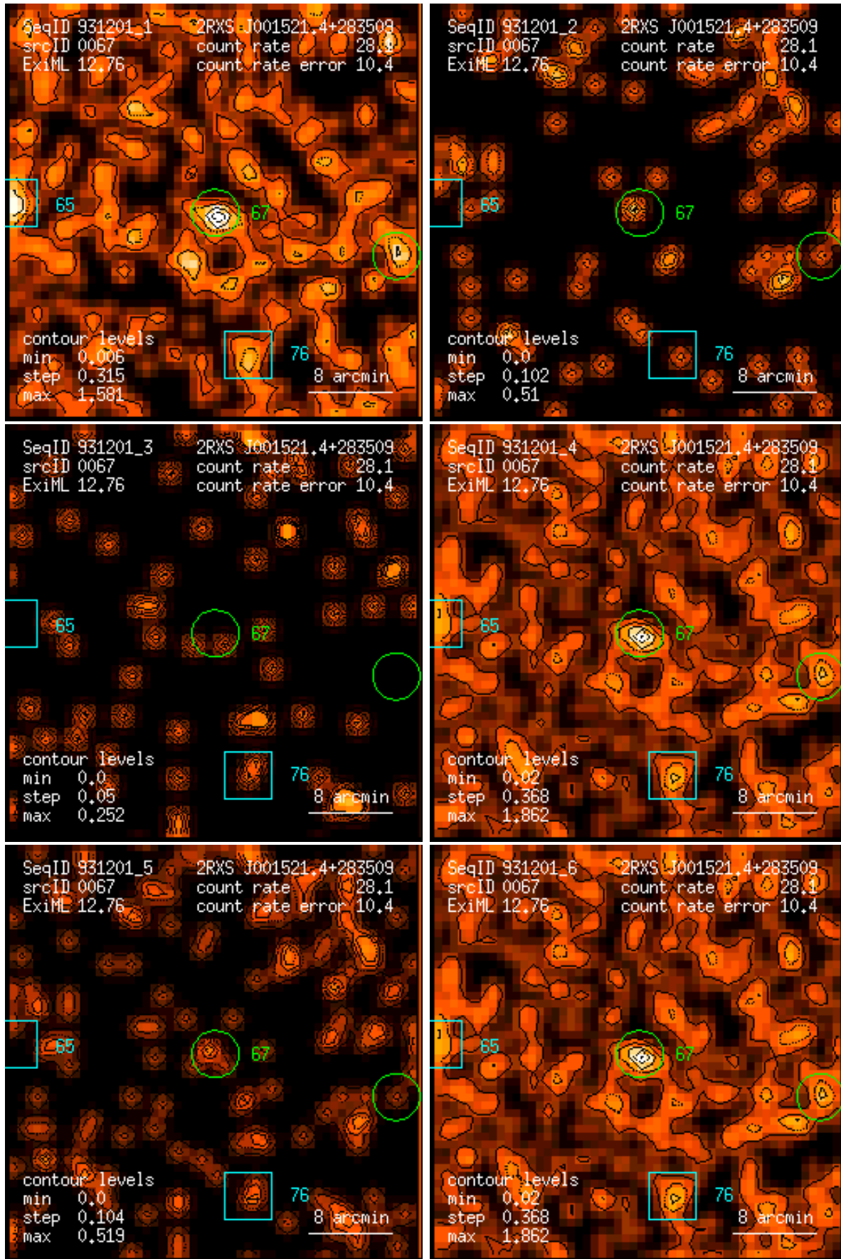
Figure 67: RASS 931201: detection 0067: band rate images, Gaussian filter: (1) PSPC channels 11 – 41, (2) 52 – 90, (3) 91 – 201, (4) 11 – 235, (5) 52 – 201, (6) 11 – 201. Broad band rates in counts/ks. Band rate contour levels in counts/ks/arcmin 2 .
