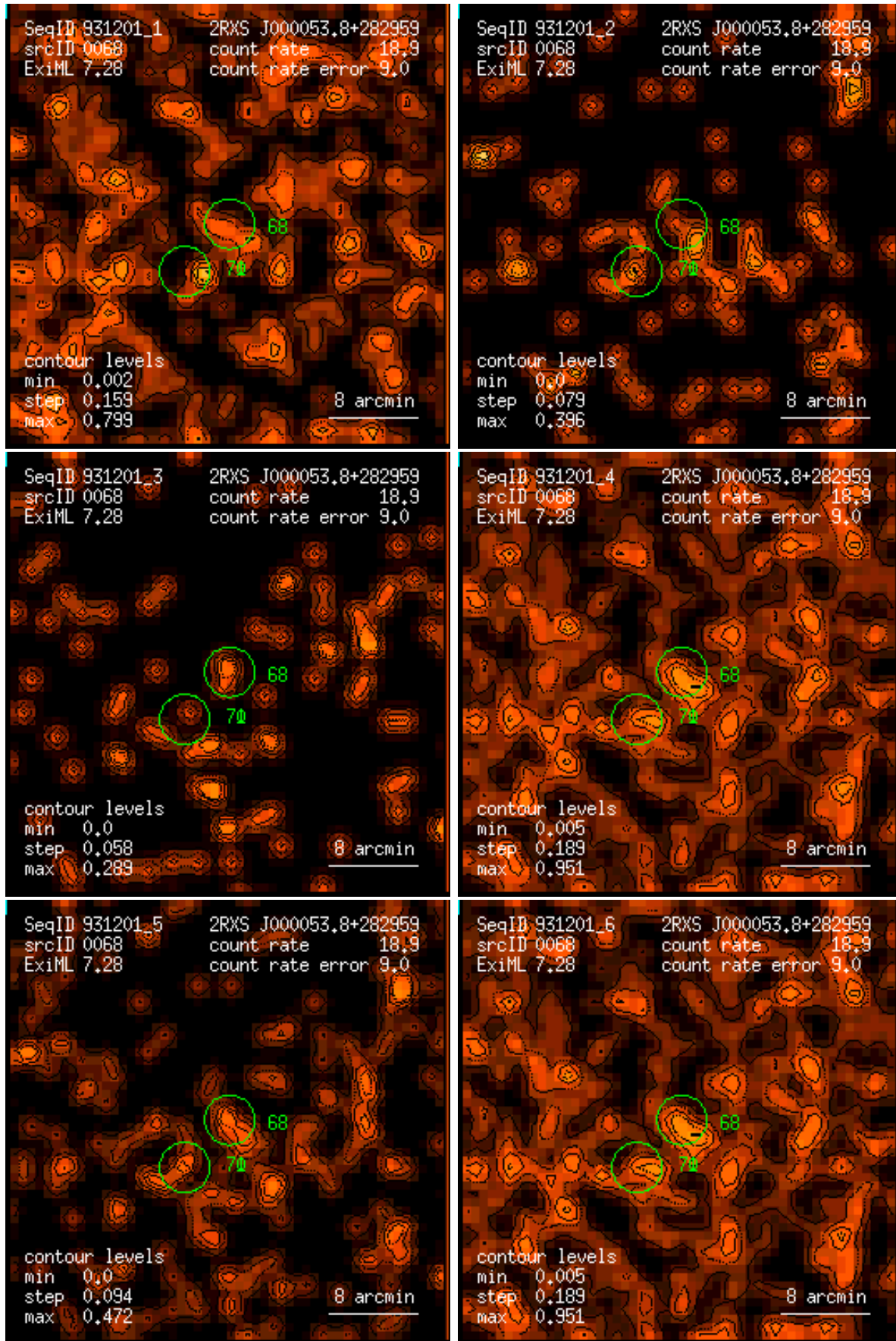
Figure 68: RASS 931201: detection 0068: band rate images, Gaussian filter: (1) PSPC channels 11 – 41, (2) 52 – 90, (3) 91 – 201, (4) 11 – 235, (5) 52 – 201, (6) 11 – 201. Broad band rates in counts/ks. Band rate contour levels in counts/ks/arcmin 2 .
