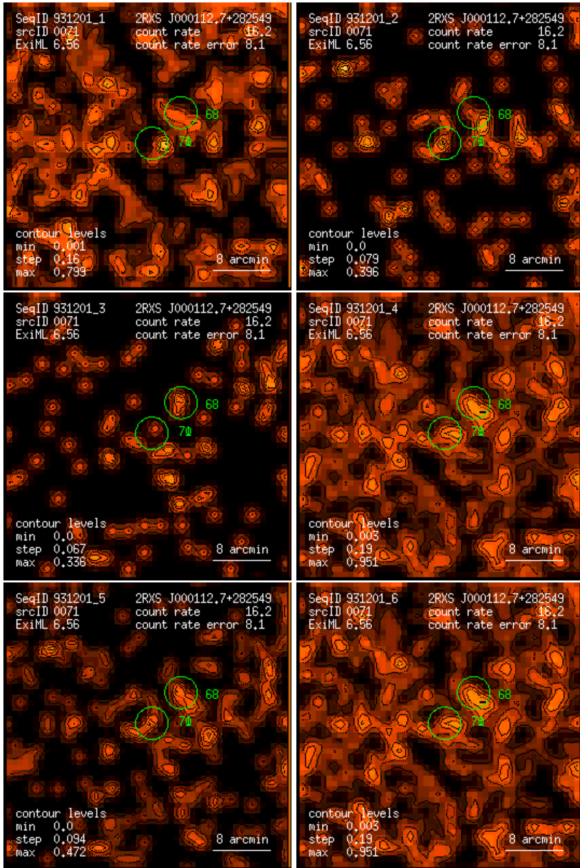
Figure 71: RASS 931201: detection 0071: band rate images, Gaussian filter: (1) PSPC channels 11 – 41, (2) 52 – 90, (3) 91 – 201, (4) 11 – 235, (5) 52 – 201, (6) 11 – 201. Broad band rates in counts/ks. Band rate contour levels in counts/ks/arcmin 2 .
