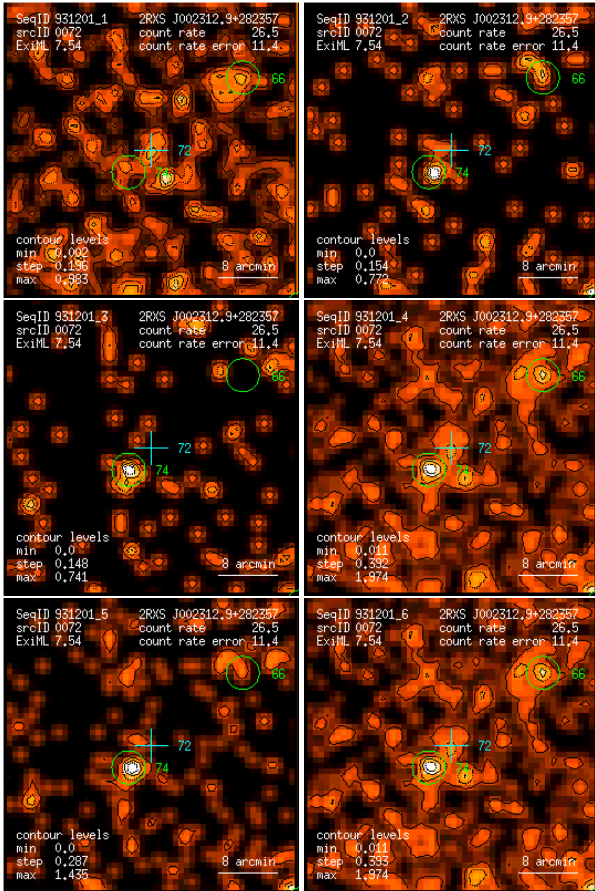
Figure 72: RASS 931201: detection 0072: band rate images, Gaussian filter: (1) PSPC channels 11 – 41, (2) 52 – 90, (3) 91 – 201, (4) 11 – 235, (5) 52 – 201, (6) 11 – 201. Broad band rates in counts/ks. Band rate contour levels in counts/ks/arcmin 2 .
