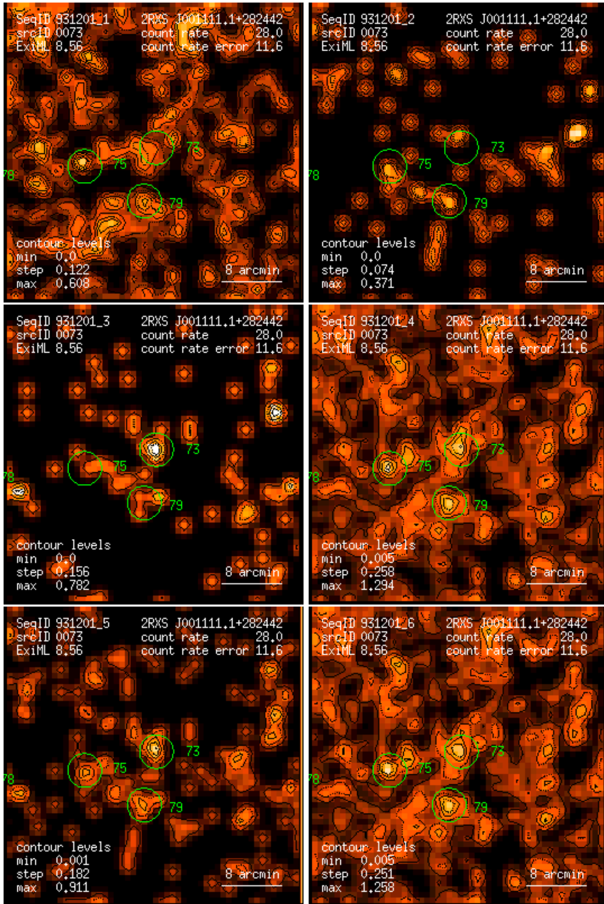
Figure 73: RASS 931201: detection 0073: band rate images, Gaussian filter: (1) PSPC channels 11 – 41, (2) 52 – 90, (3) 91 – 201, (4) 11 – 235, (5) 52 – 201, (6) 11 – 201. Broad band rates in counts/ks. Band rate contour levels in counts/ks/arcmin 2 .
