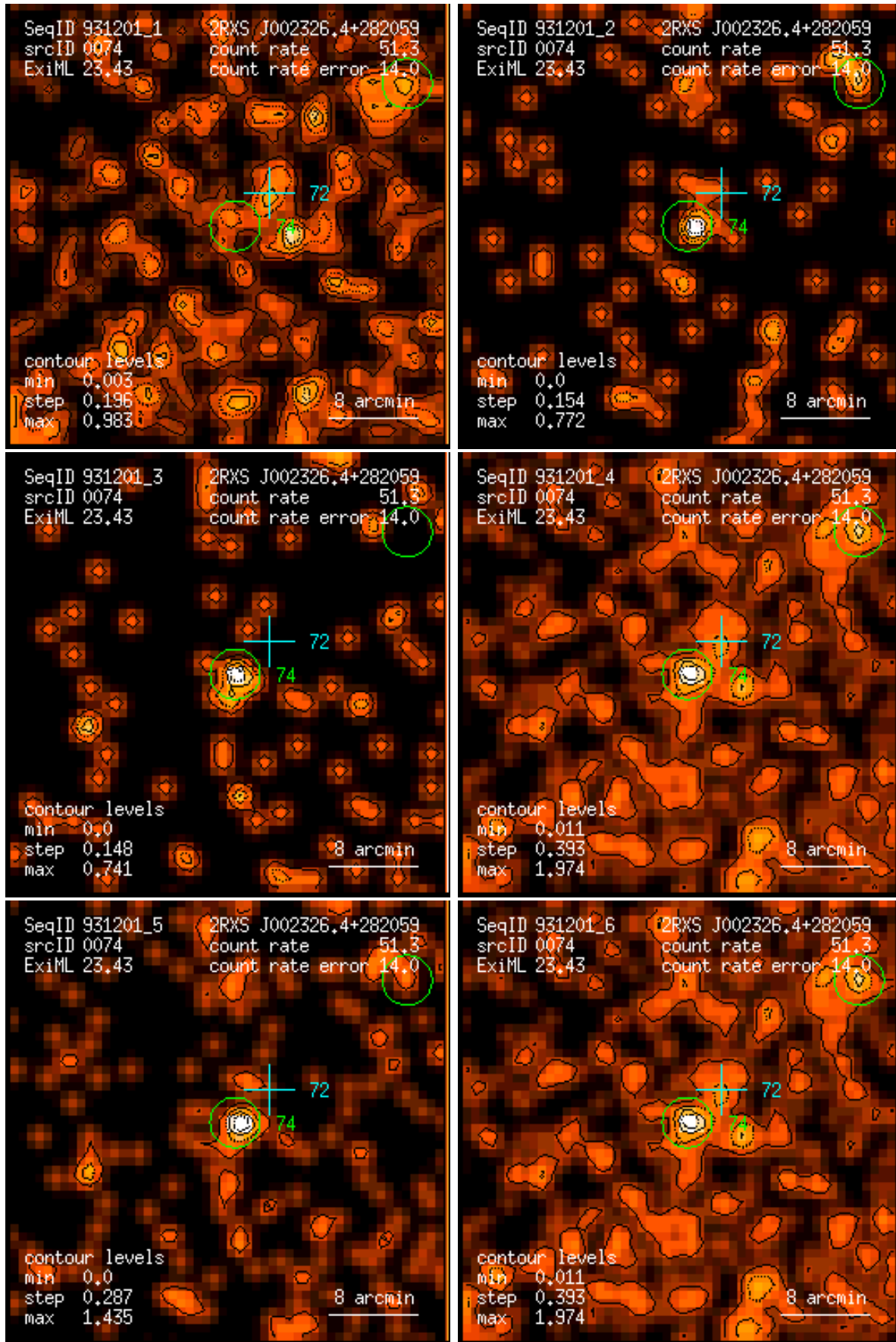
Figure 74: RASS 931201: detection 0074: band rate images, Gaussian filter: (1) PSPC channels 11 – 41, (2) 52 – 90, (3) 91 – 201, (4) 11 – 235, (5) 52 – 201, (6) 11 – 201. Broad band rates in counts/ks. Band rate contour levels in counts/ks/arcmin 2 .
