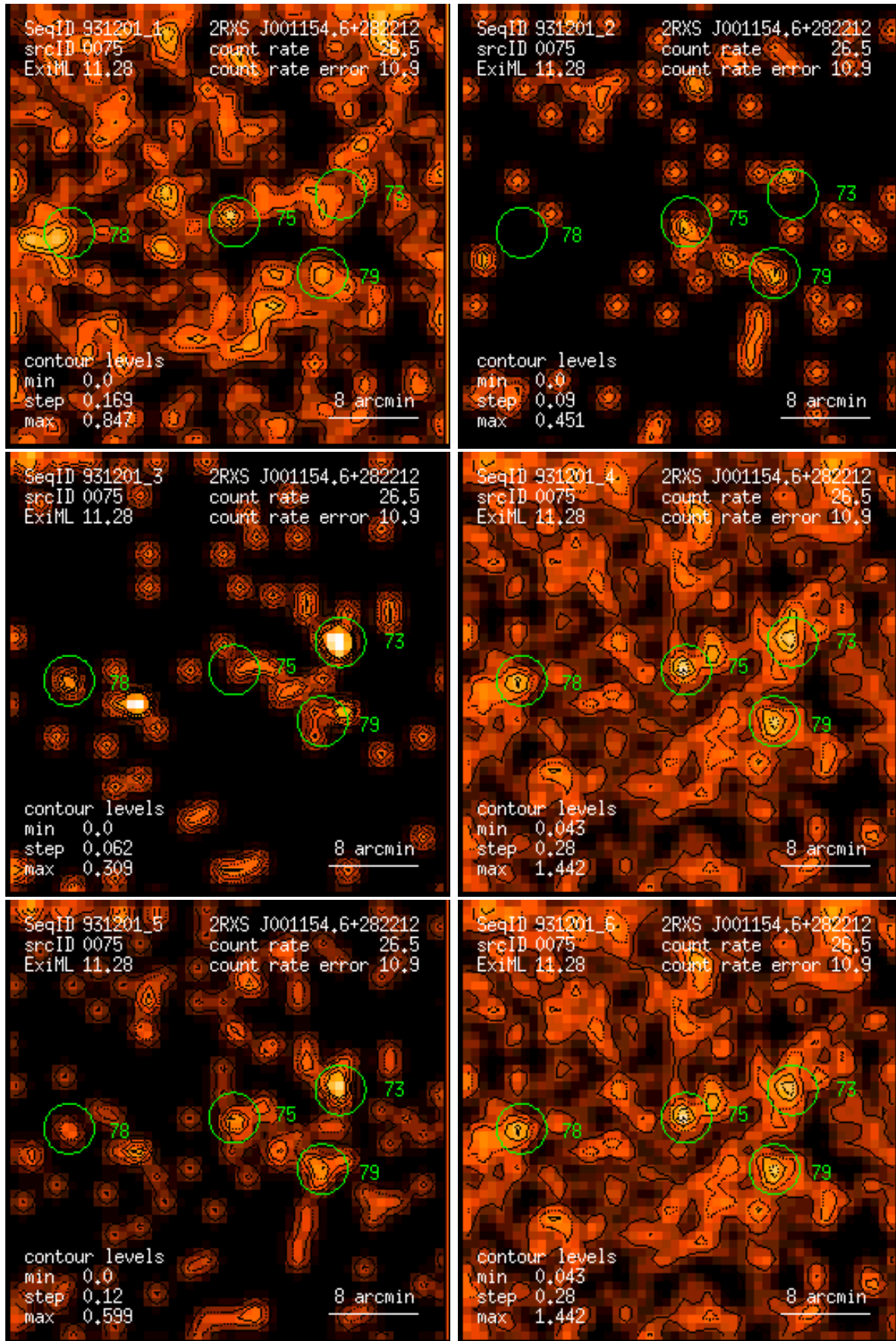
Figure 75: RASS 931201: detection 0075: band rate images, Gaussian filter: (1) PSPC channels 11 – 41, (2) 52 – 90, (3) 91 – 201, (4) 11 – 235, (5) 52 – 201, (6) 11 – 201. Broad band rates in counts/ks. Band rate contour levels in counts/ks/arcmin 2 .
