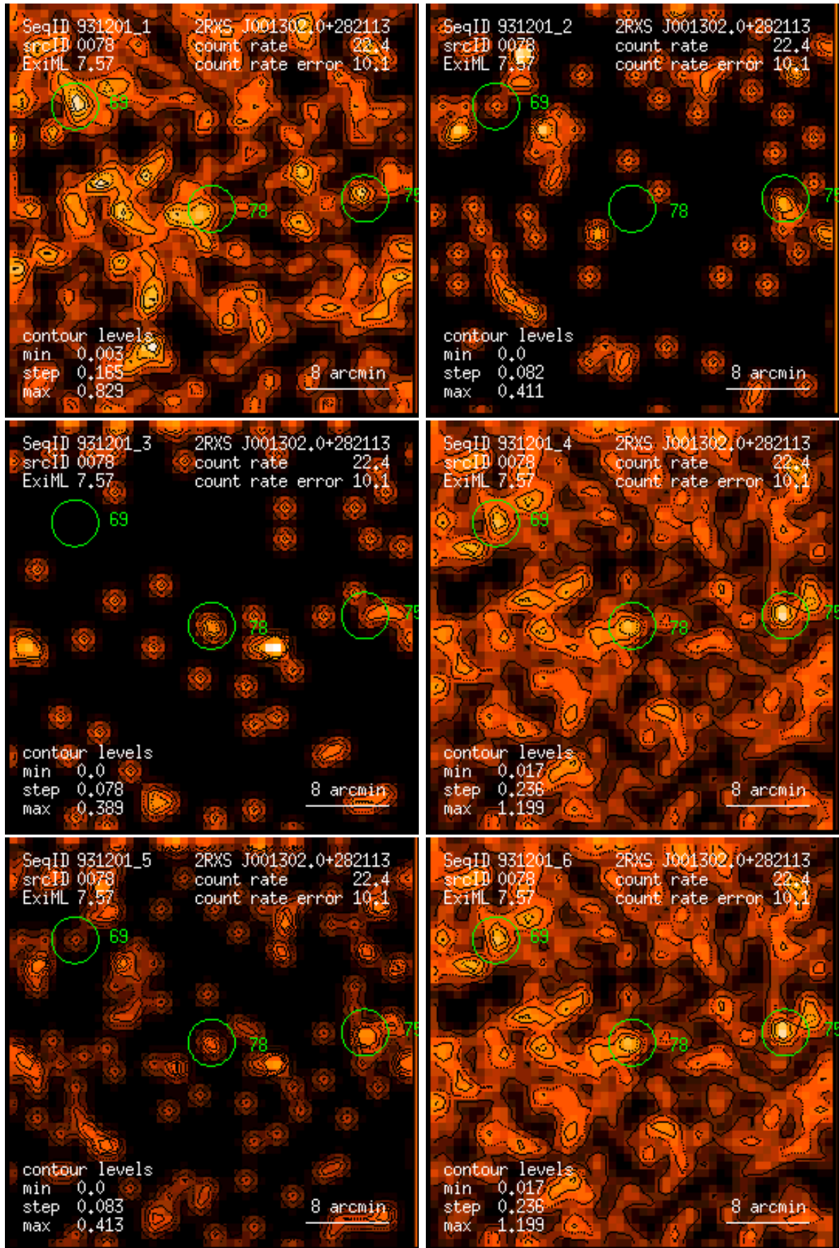
Figure 78: RASS 931201: detection 0078: band rate images, Gaussian filter: (1) PSPC channels 11 – 41, (2) 52 – 90, (3) 91 – 201, (4) 11 – 235, (5) 52 – 201, (6) 11 – 201. Broad band rates in counts/ks. Band rate contour levels in counts/ks/arcmin 2 .
