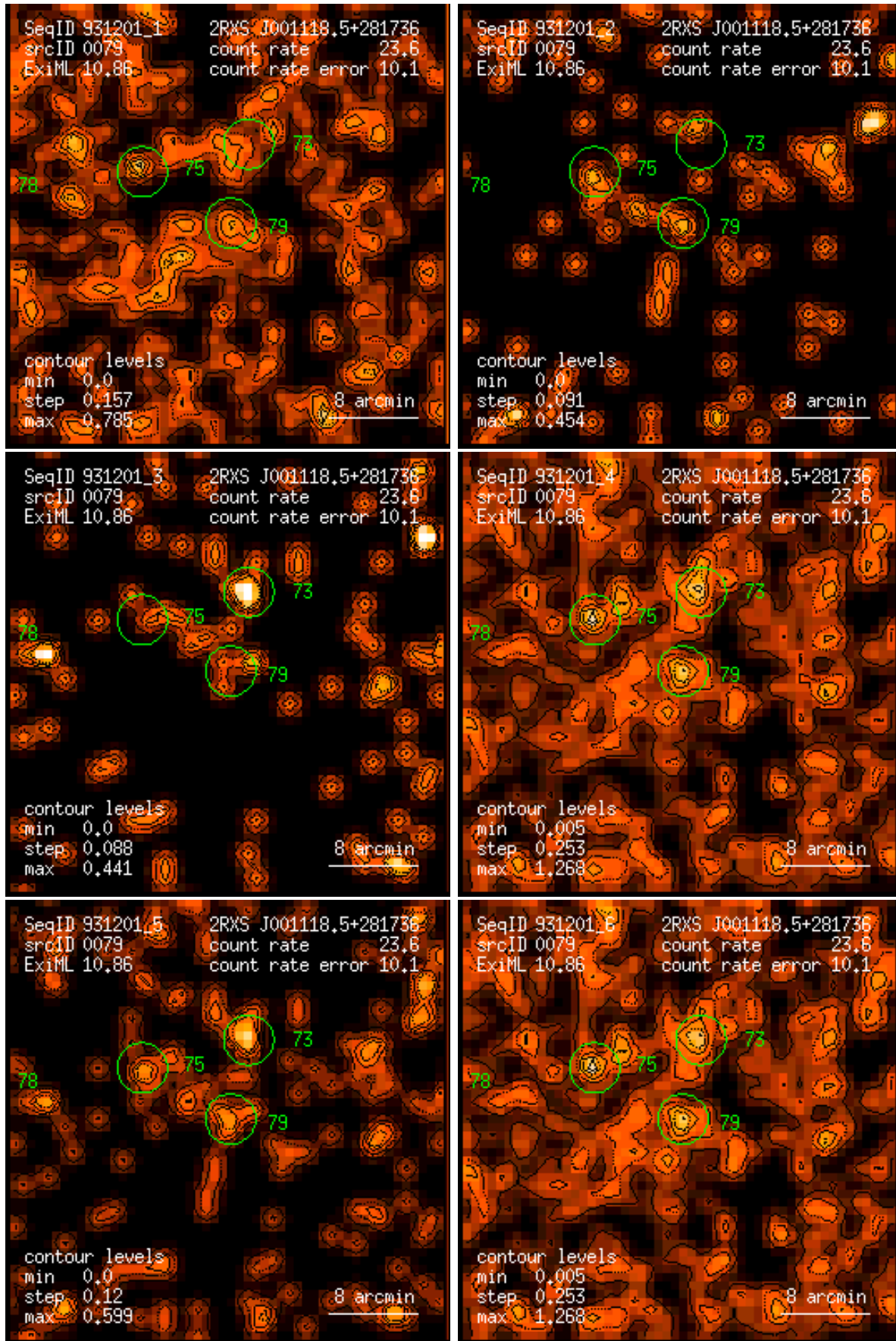
Figure 79: RASS 931201: detection 0079: band rate images, Gaussian filter: (1) PSPC channels 11 – 41, (2) 52 – 90, (3) 91 – 201, (4) 11 – 235, (5) 52 – 201, (6) 11 – 201. Broad band rates in counts/ks. Band rate contour levels in counts/ks/arcmin 2 .
