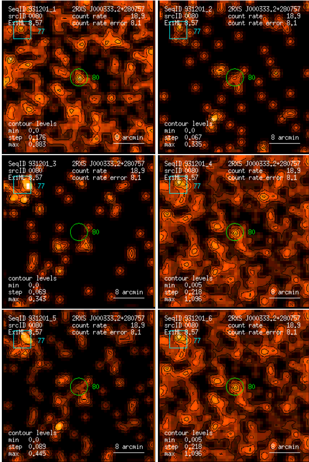
Figure 80: RASS 931201: detection 0080: band rate images, Gaussian filter: (1) PSPC channels 11 – 41, (2) 52 – 90, (3) 91 – 201, (4) 11 – 235, (5) 52 – 201, (6) 11 – 201. Broad band rates in counts/ks. Band rate contour levels in counts/ks/arcmin 2 .
