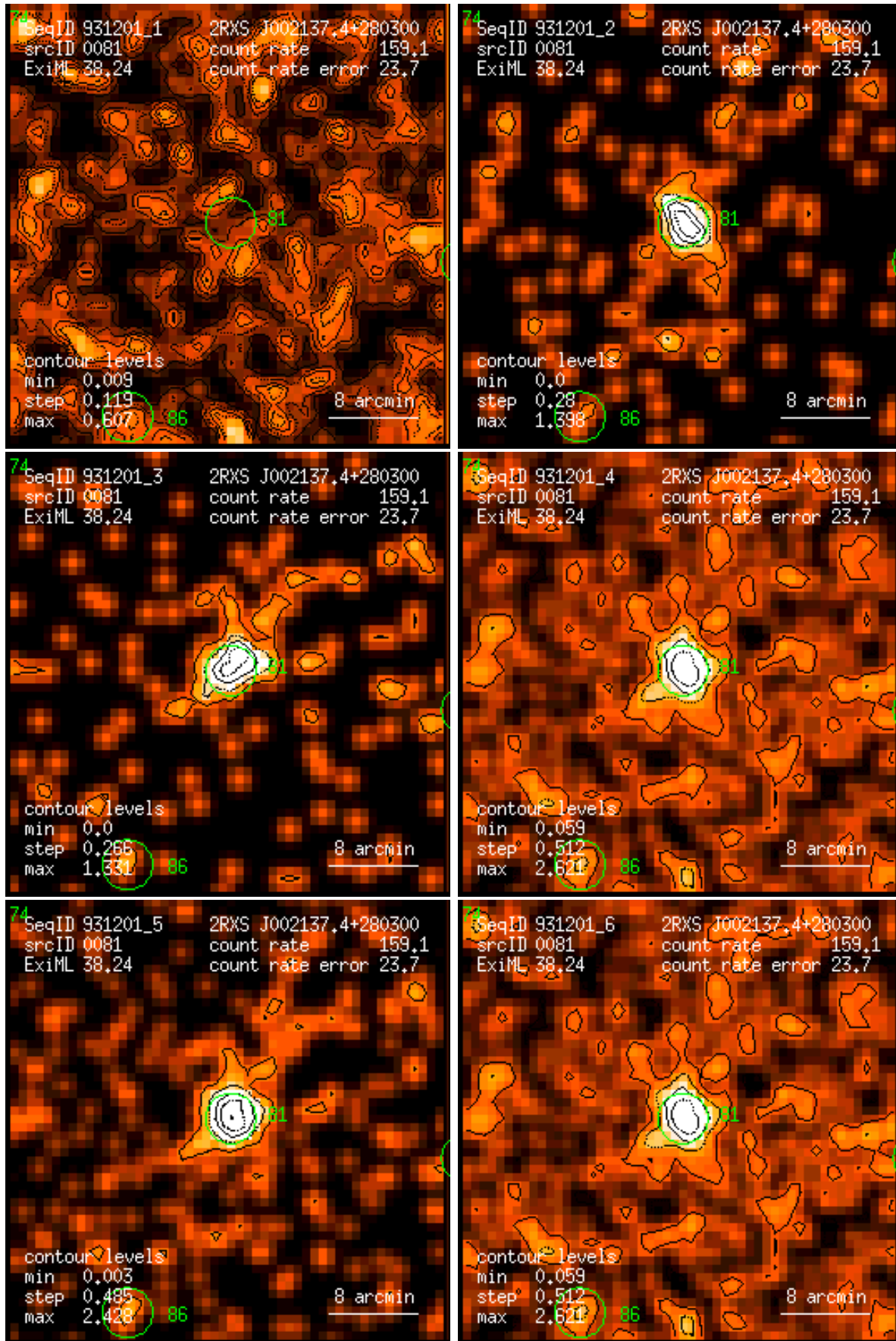
Figure 81: RASS 931201: detection 0081: band rate images, Gaussian filter: (1) PSPC channels 11 – 41, (2) 52 – 90, (3) 91 – 201, (4) 11 – 235, (5) 52 – 201, (6) 11 – 201. Broad band rates in counts/ks. Band rate contour levels in counts/ks/arcmin 2 .
