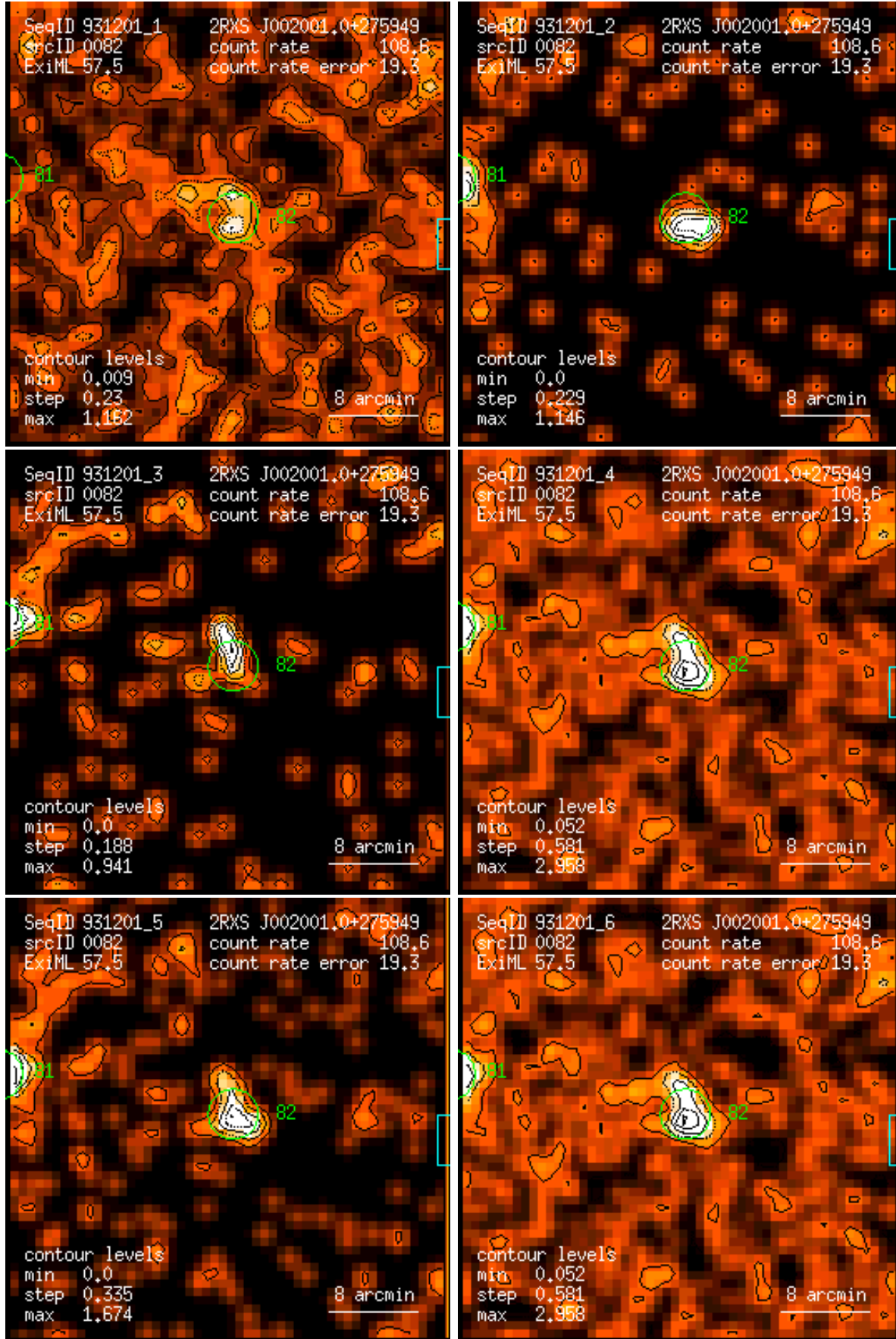
Figure 82: RASS 931201: detection 0082: band rate images, Gaussian filter: (1) PSPC channels 11 – 41, (2) 52 – 90, (3) 91 – 201, (4) 11 – 235, (5) 52 – 201, (6) 11 – 201. Broad band rates in counts/ks. Band rate contour levels in counts/ks/arcmin 2 .
