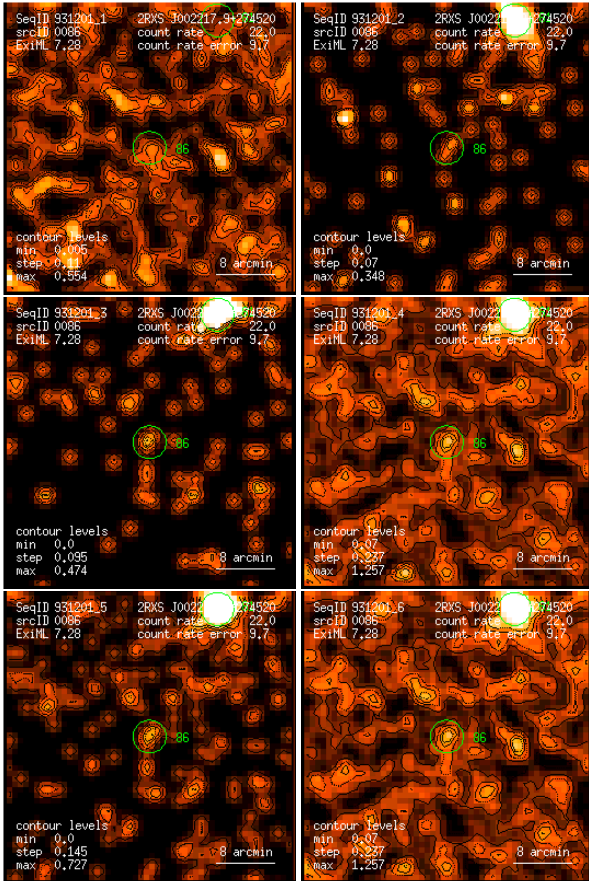
Figure 86: RASS 931201: detection 0086: band rate images, Gaussian filter: (1) PSPC channels 11 – 41, (2) 52 – 90, (3) 91 – 201, (4) 11 – 235, (5) 52 – 201, (6) 11 – 201. Broad band rates in counts/ks. Band rate contour levels in counts/ks/arcmin 2 .
