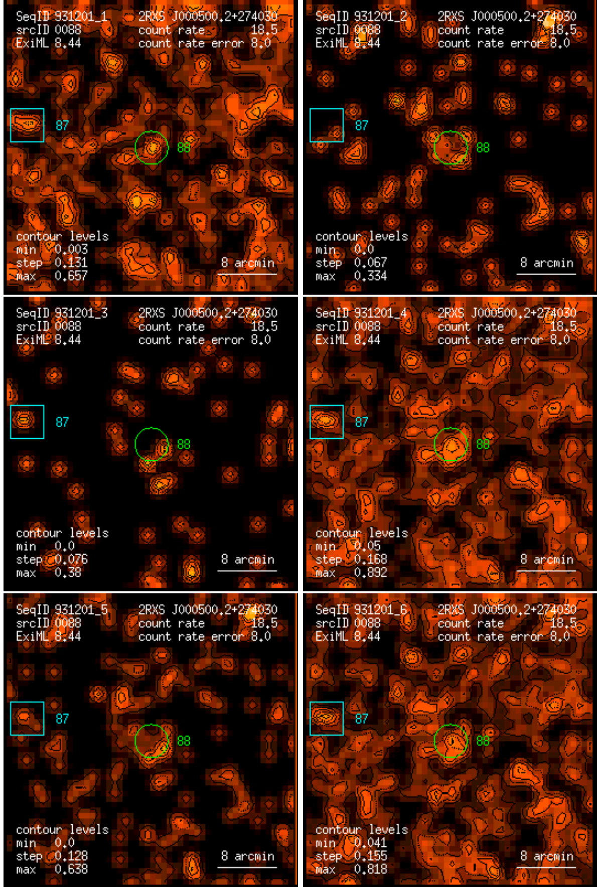
Figure 88: RASS 931201: detection 0088: band rate images, Gaussian filter: (1) PSPC channels 11 – 41, (2) 52 – 90, (3) 91 – 201, (4) 11 – 235, (5) 52 – 201, (6) 11 – 201. Broad band rates in counts/ks. Band rate contour levels in counts/ks/arcmin 2 .
