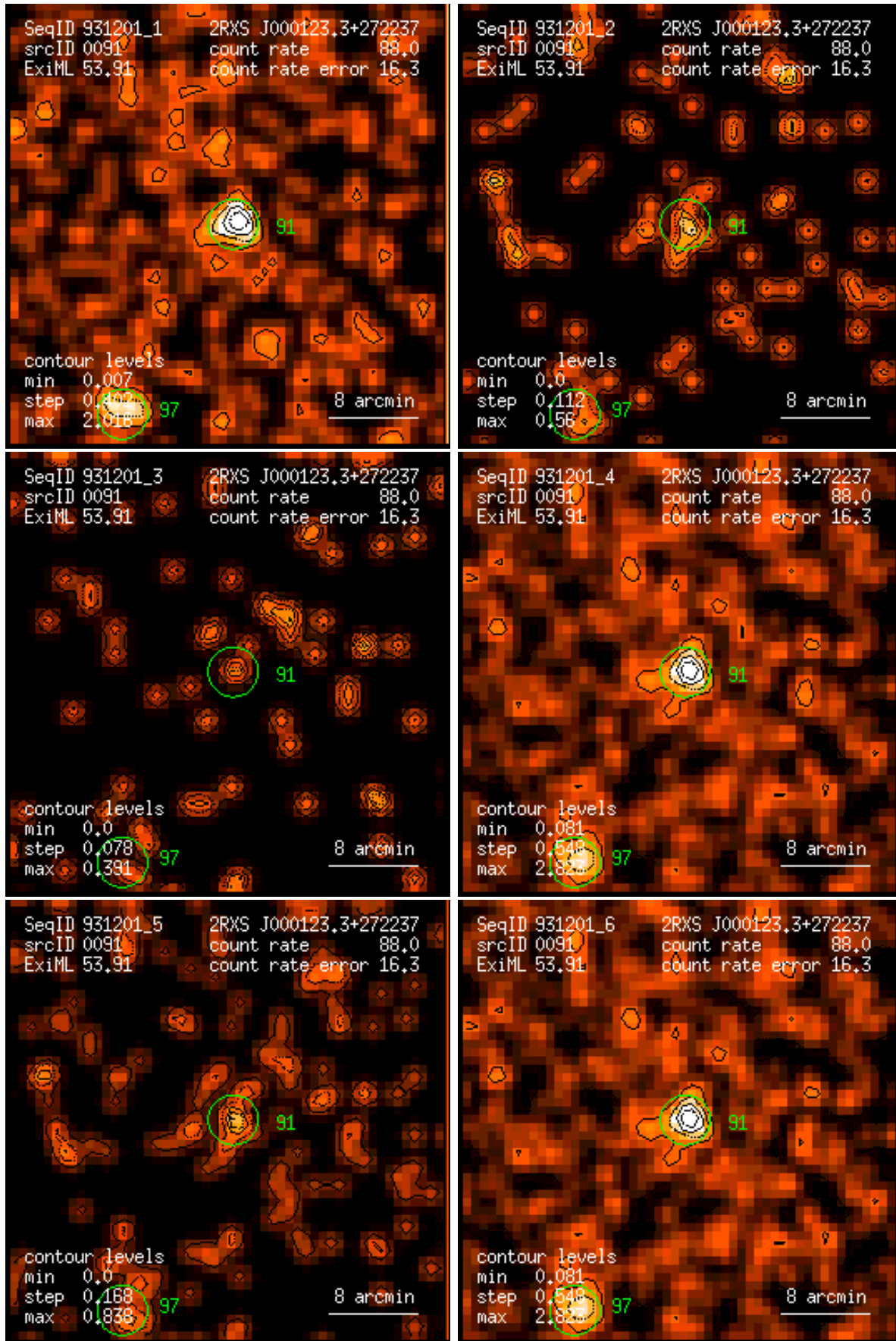
Figure 91: RASS 931201: detection 0091: band rate images, Gaussian filter: (1) PSPC channels 11 – 41, (2) 52 – 90, (3) 91 – 201, (4) 11 – 235, (5) 52 – 201, (6) 11 – 201. Broad band rates in counts/ks. Band rate contour levels in counts/ks/arcmin 2 .
