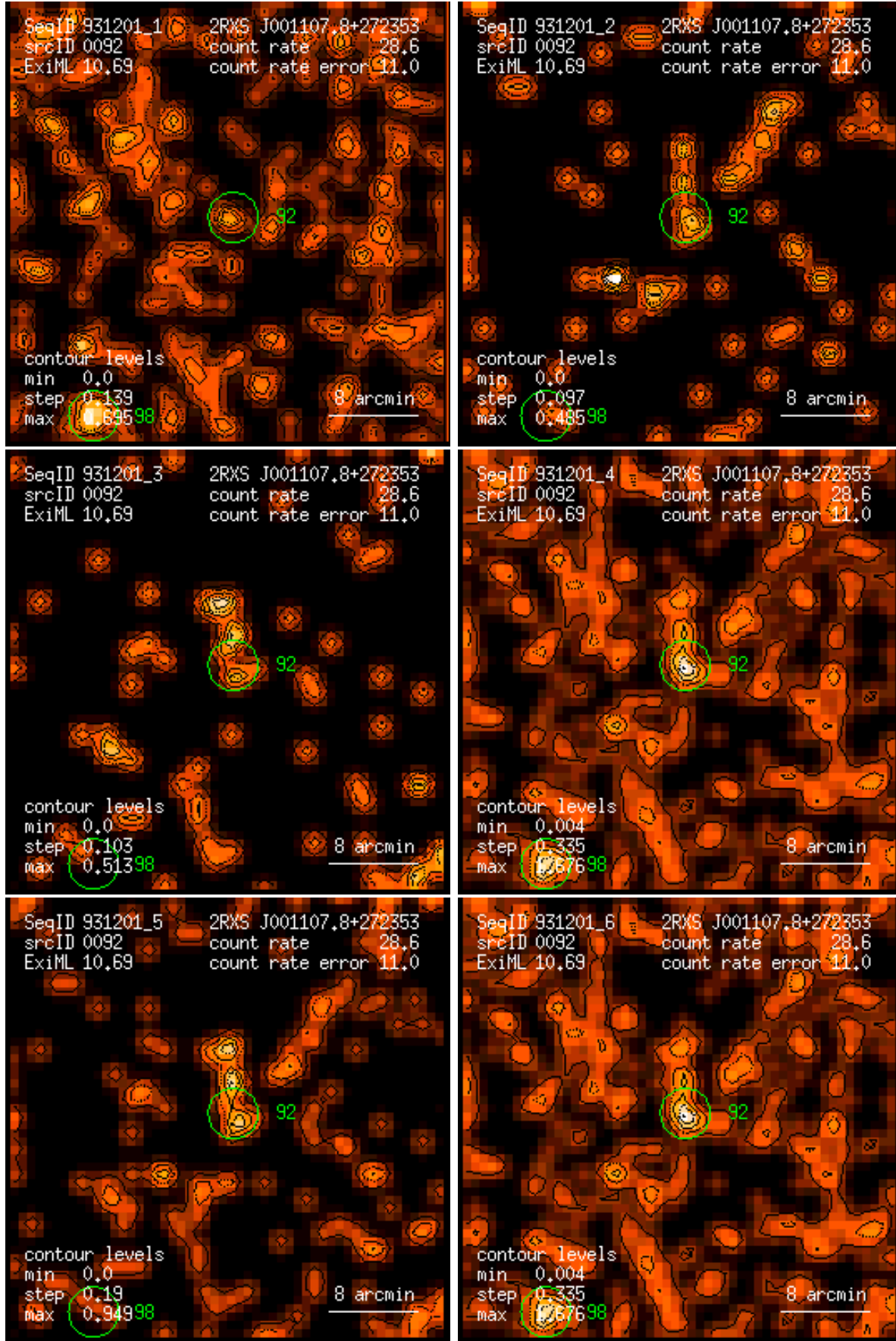
Figure 92: RASS 931201: detection 0092: band rate images, Gaussian filter: (1) PSPC channels 11 – 41, (2) 52 – 90, (3) 91 – 201, (4) 11 – 235, (5) 52 – 201, (6) 11 – 201. Broad band rates in counts/ks. Band rate contour levels in counts/ks/arcmin 2 .
