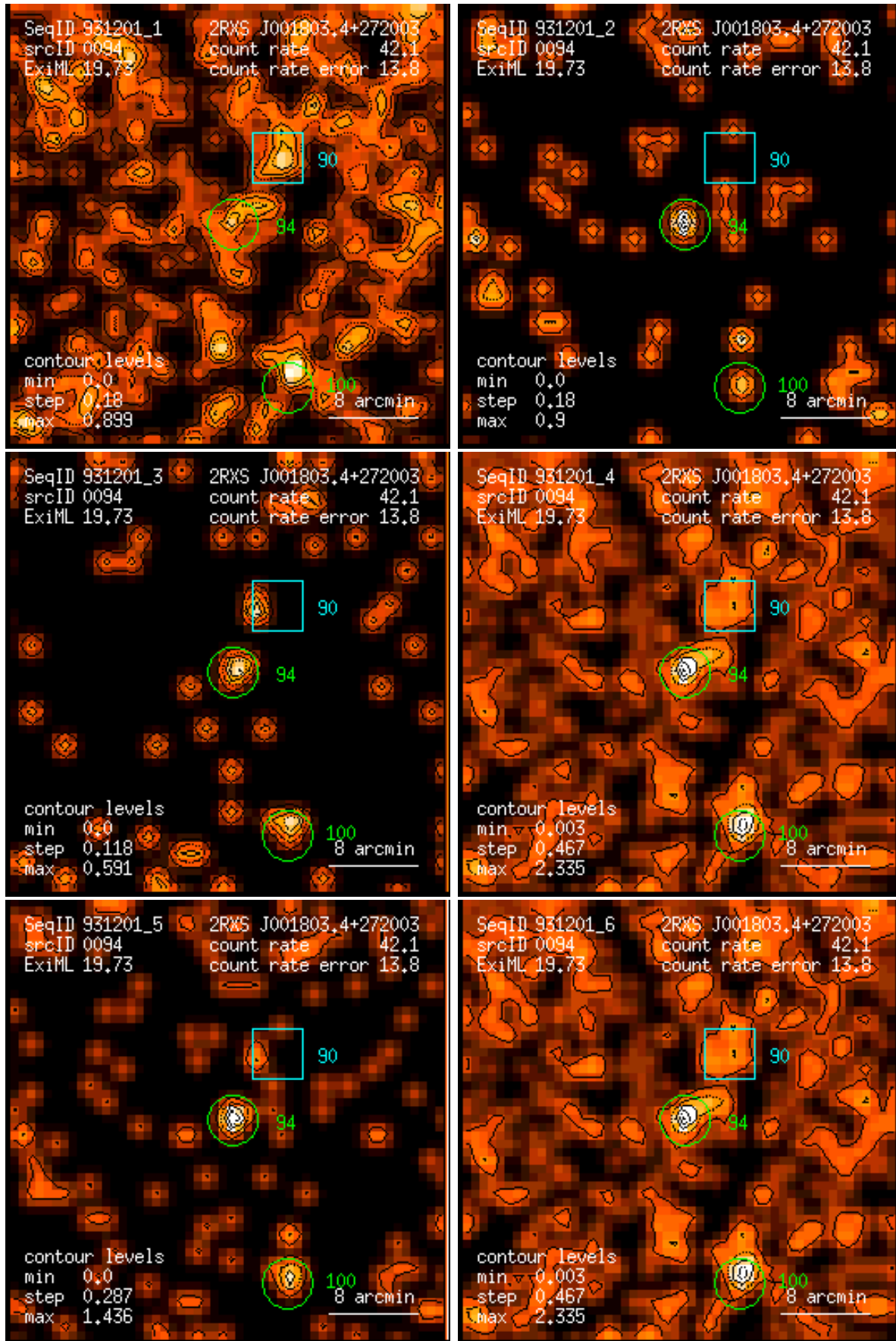
Figure 94: RASS 931201: detection 0094: band rate images, Gaussian filter: (1) PSPC channels 11 – 41, (2) 52 – 90, (3) 91 – 201, (4) 11 – 235, (5) 52 – 201, (6) 11 – 201. Broad band rates in counts/ks. Band rate contour levels in counts/ks/arcmin 2 .
