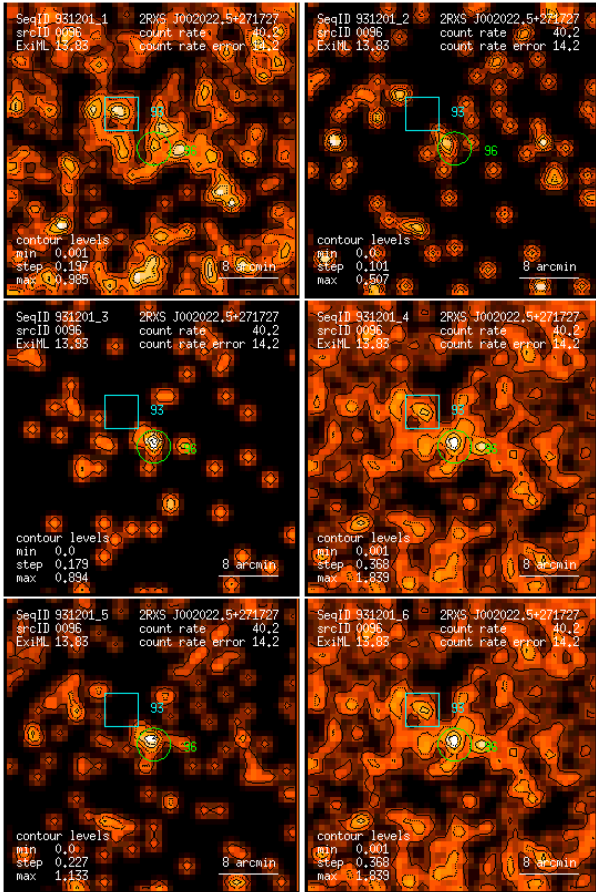
Figure 96: RASS 931201: detection 0096: band rate images, Gaussian filter: (1) PSPC channels 11 – 41, (2) 52 – 90, (3) 91 – 201, (4) 11 – 235, (5) 52 – 201, (6) 11 – 201. Broad band rates in counts/ks. Band rate contour levels in counts/ks/arcmin 2 .
