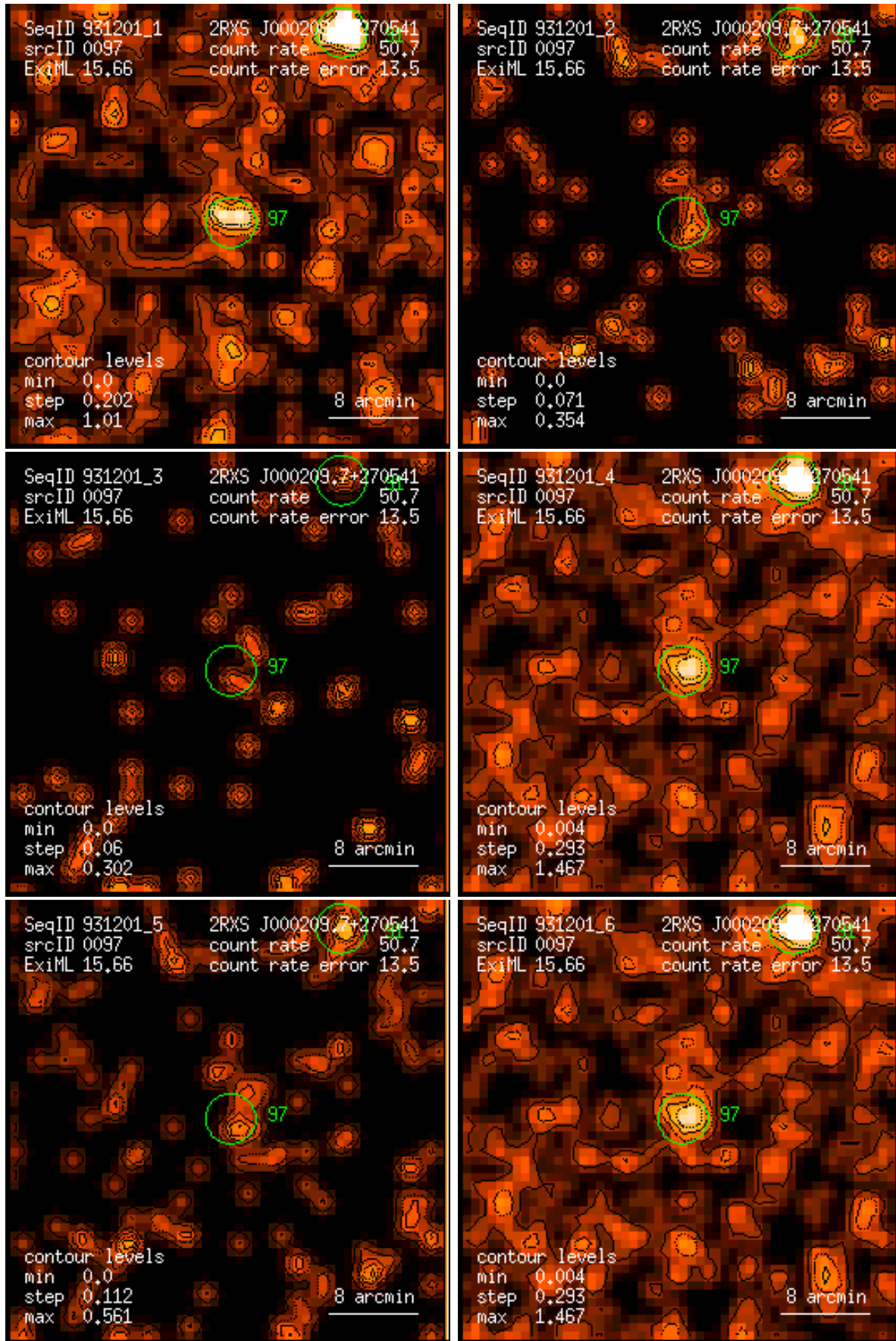
Figure 97: RASS 931201: detection 0097: band rate images, Gaussian filter: (1) PSPC channels 11 – 41, (2) 52 – 90, (3) 91 – 201, (4) 11 – 235, (5) 52 – 201, (6) 11 – 201. Broad band rates in counts/ks. Band rate contour levels in counts/ks/arcmin 2 .
