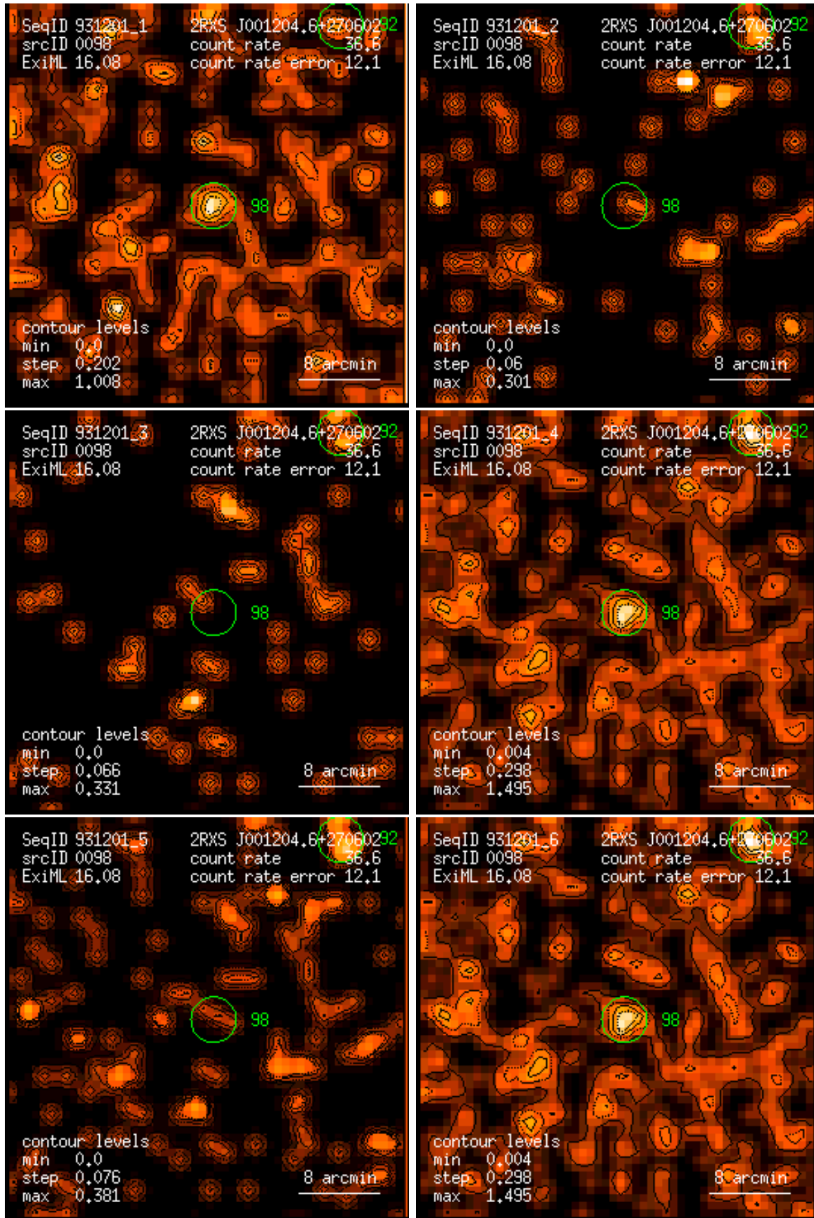
Figure 98: RASS 931201: detection 0098: band rate images, Gaussian filter: (1) PSPC channels 11 – 41, (2) 52 – 90, (3) 91 – 201, (4) 11 – 235, (5) 52 – 201, (6) 11 – 201. Broad band rates in counts/ks. Band rate contour levels in counts/ks/arcmin 2 .
