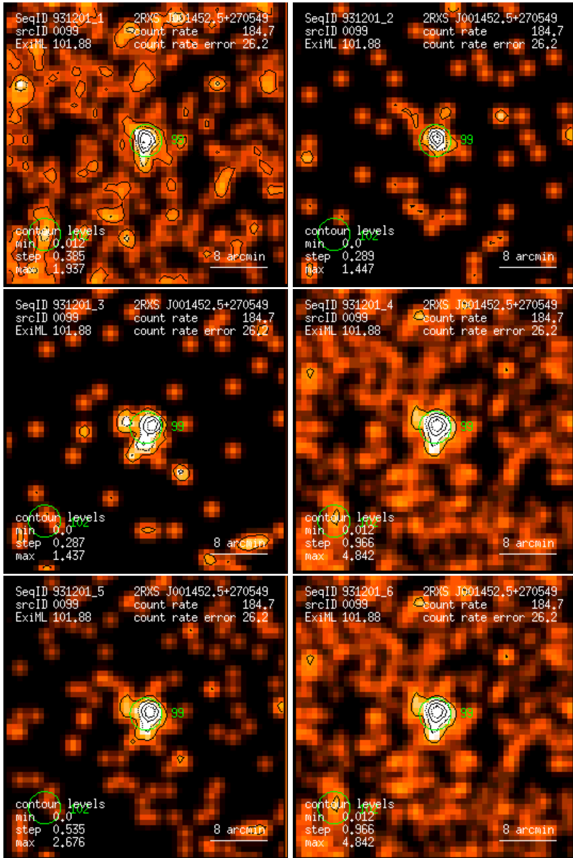
Figure 99: RASS 931201: detection 0099: band rate images, Gaussian filter: (1) PSPC channels 11 – 41, (2) 52 – 90, (3) 91 – 201, (4) 11 – 235, (5) 52 – 201, (6) 11 – 201. Broad band rates in counts/ks. Band rate contour levels in counts/ks/arcmin 2 .
