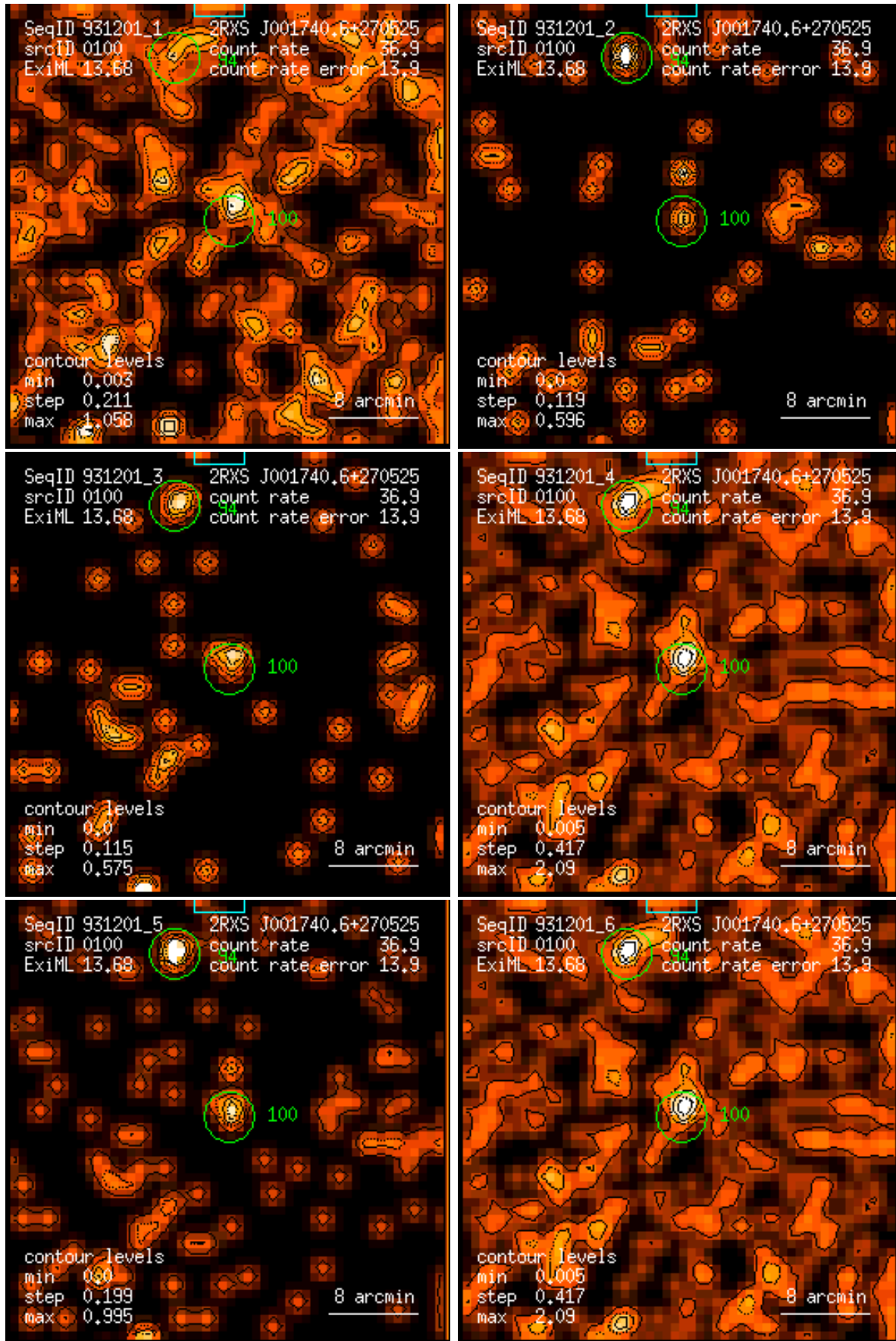
Figure 100: RASS 931201: detection 0100: band rate images, Gaussian filter: (1) PSPC channels 11 – 41, (2) 52 – 90, (3) 91 – 201, (4) 11 – 235, (5) 52 – 201, (6) 11 – 201. Broad band rates in counts/ks. Band rate contour levels in counts/ks/arcmin 2 .
