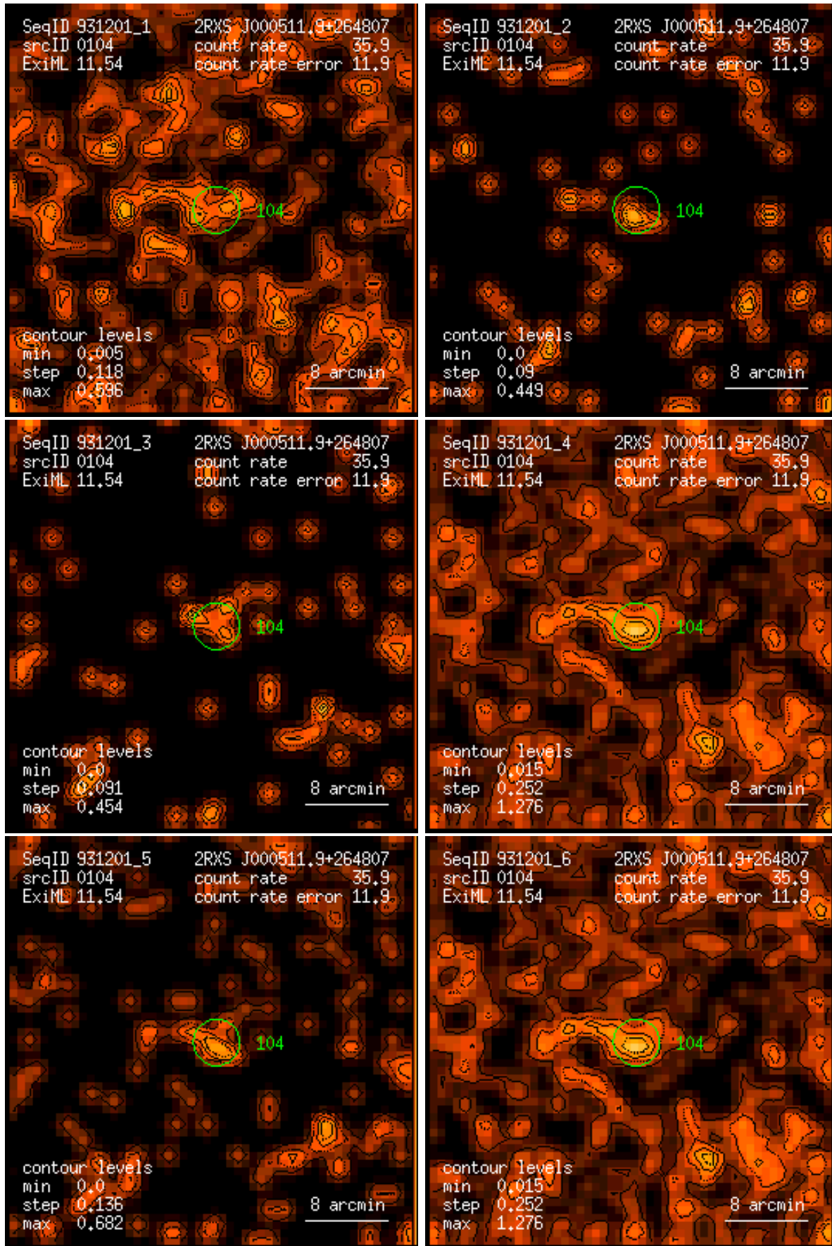
Figure 104: RASS 931201: detection 0104: band rate images, Gaussian filter: (1) PSPC channels 11 – 41, (2) 52 – 90, (3) 91 – 201, (4) 11 – 235, (5) 52 – 201, (6) 11 – 201. Broad band rates in counts/ks. Band rate contour levels in counts/ks/arcmin 2 .
