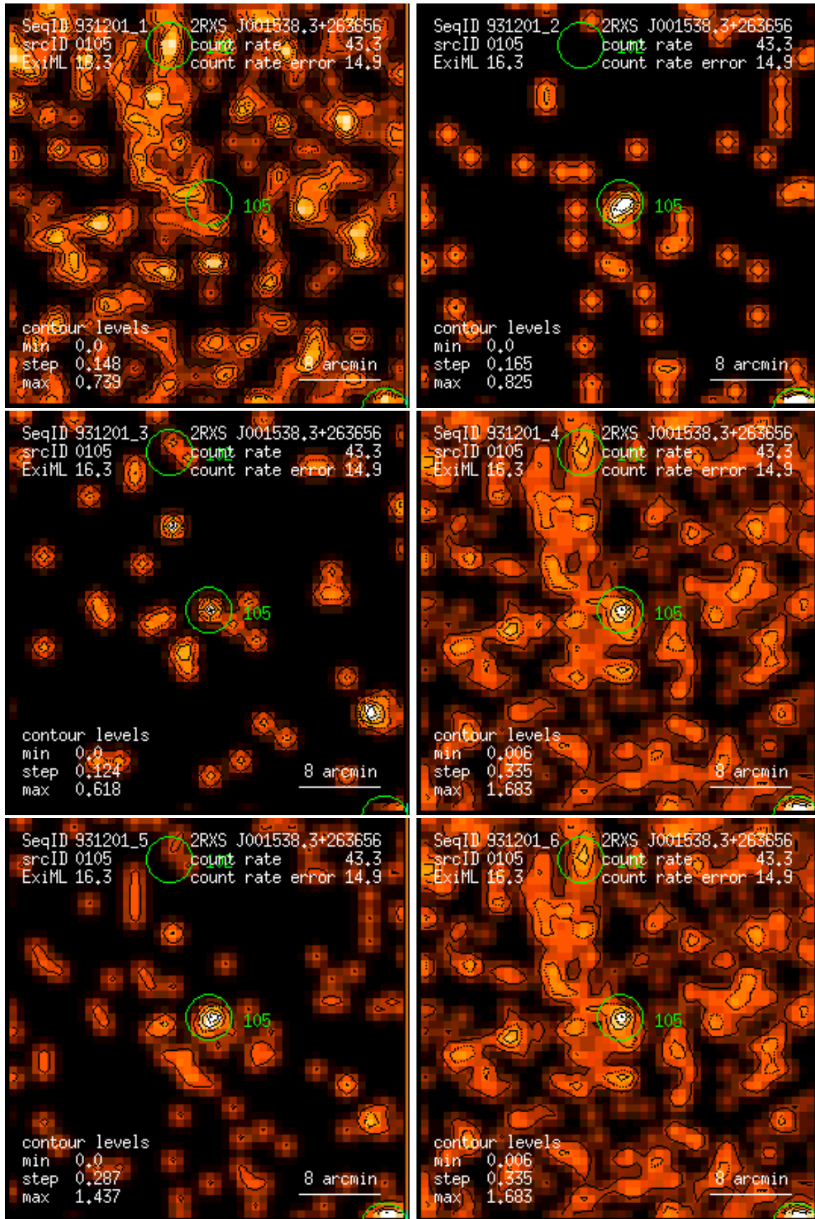
Figure 105: RASS 931201: detection 0105: band rate images, Gaussian filter: (1) PSPC channels 11 – 41, (2) 52 – 90, (3) 91 – 201, (4) 11 – 235, (5) 52 – 201, (6) 11 – 201. Broad band rates in counts/ks. Band rate contour levels in counts/ks/arcmin 2 .
