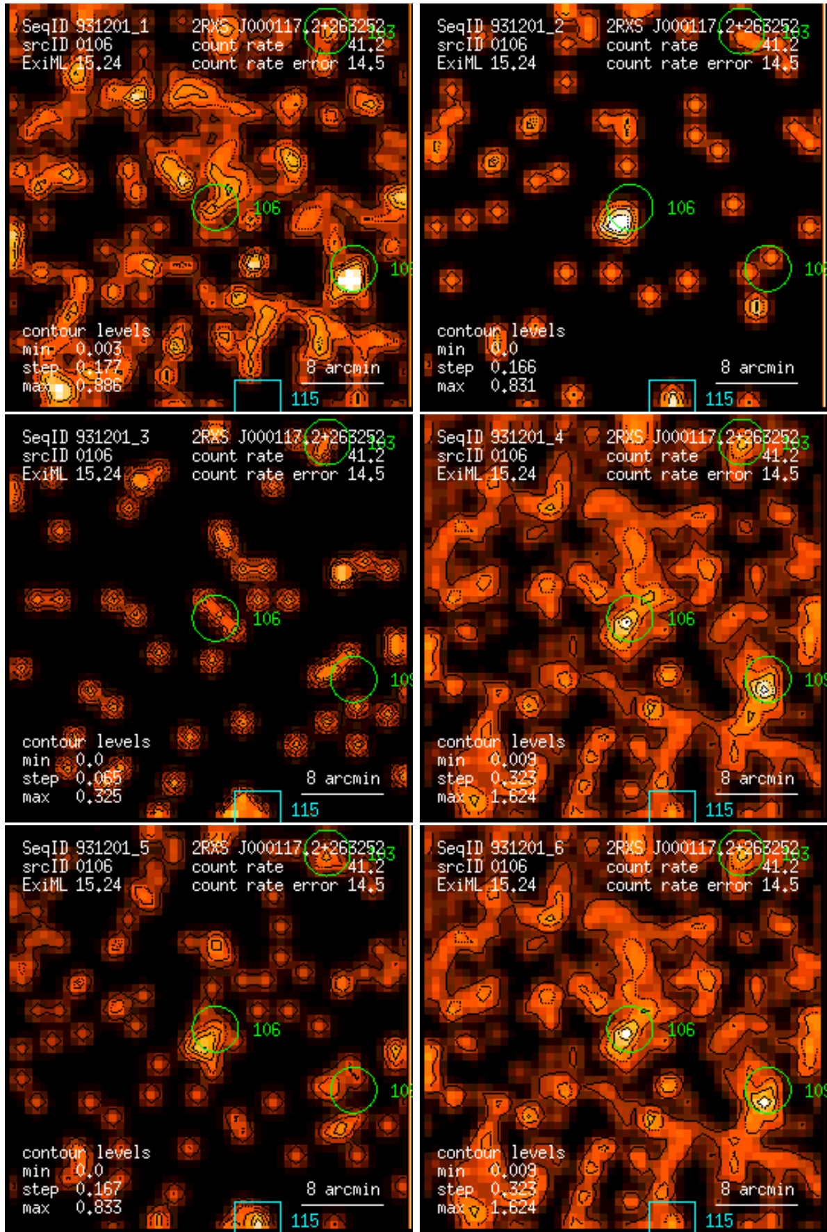
Figure 106: RASS 931201: detection 0106: band rate images, Gaussian filter: (1) PSPC channels 11 – 41, (2) 52 – 90, (3) 91 – 201, (4) 11 – 235, (5) 52 – 201, (6) 11 – 201. Broad band rates in counts/ks. Band rate contour levels in counts/ks/arcmin 2 .
