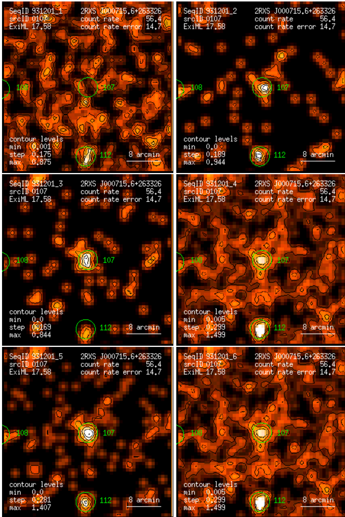
Figure 107: RASS 931201: detection 0107: band rate images, Gaussian filter: (1) PSPC channels 11 – 41, (2) 52 – 90, (3) 91 – 201, (4) 11 – 235, (5) 52 – 201, (6) 11 – 201. Broad band rates in counts/ks. Band rate contour levels in counts/ks/arcmin 2 .
