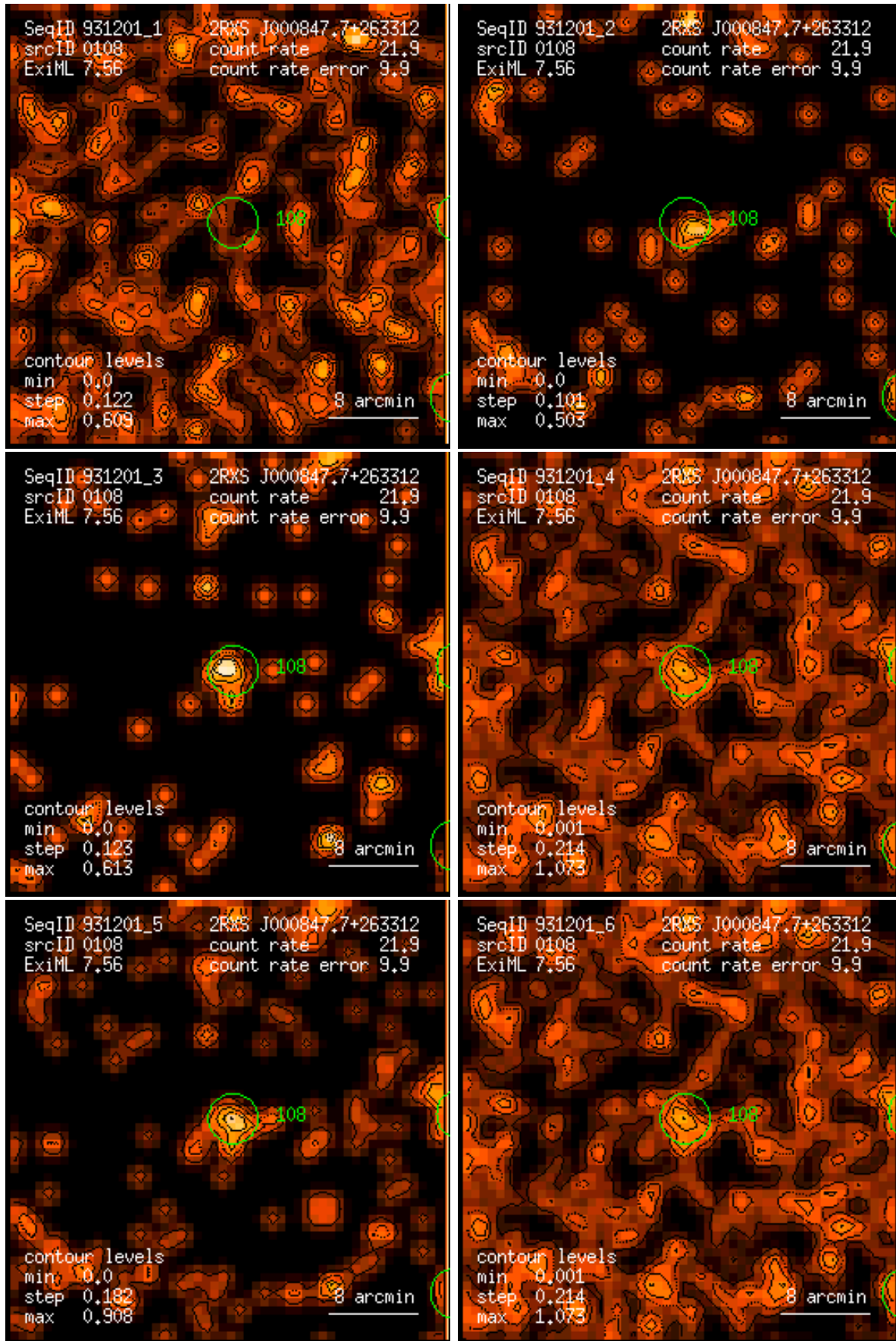
Figure 108: RASS 931201: detection 0108: band rate images, Gaussian filter: (1) PSPC channels 11 – 41, (2) 52 – 90, (3) 91 – 201, (4) 11 – 235, (5) 52 – 201, (6) 11 – 201. Broad band rates in counts/ks. Band rate contour levels in counts/ks/arcmin 2 .
