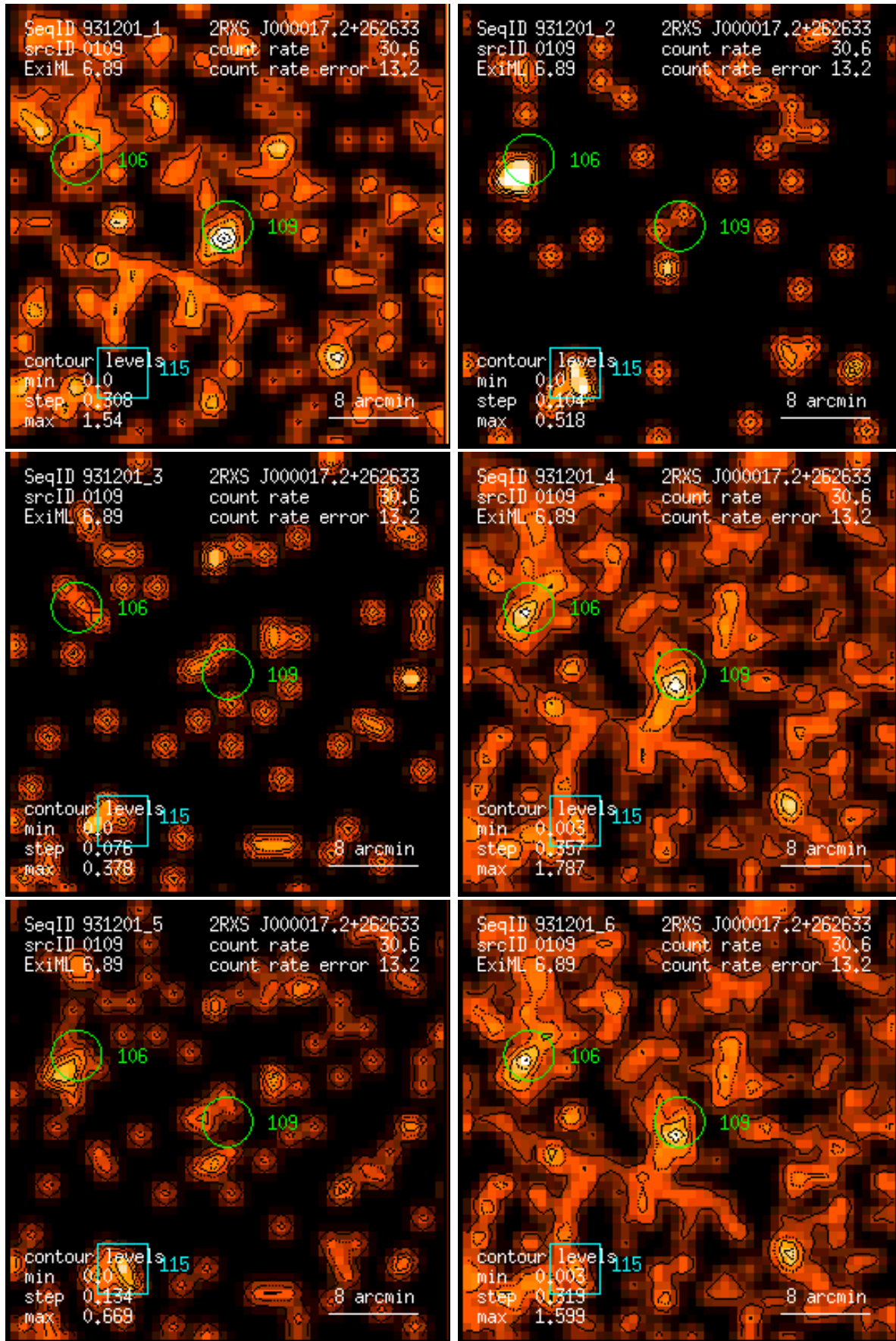
Figure 109: RASS 931201: detection 0109: band rate images, Gaussian filter: (1) PSPC channels 11 – 41, (2) 52 – 90, (3) 91 – 201, (4) 11 – 235, (5) 52 – 201, (6) 11 – 201. Broad band rates in counts/ks. Band rate contour levels in counts/ks/arcmin 2 .
