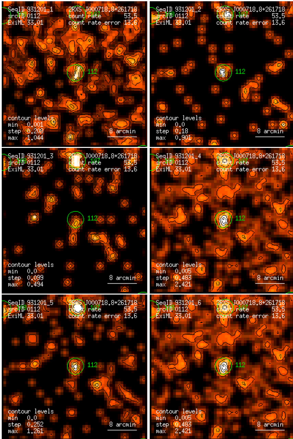
Figure 112: RASS 931201: detection 0112: band rate images, Gaussian filter: (1) PSPC channels 11 – 41, (2) 52 – 90, (3) 91 – 201, (4) 11 – 235, (5) 52 – 201, (6) 11 – 201. Broad band rates in counts/ks. Band rate contour levels in counts/ks/arcmin 2 .
