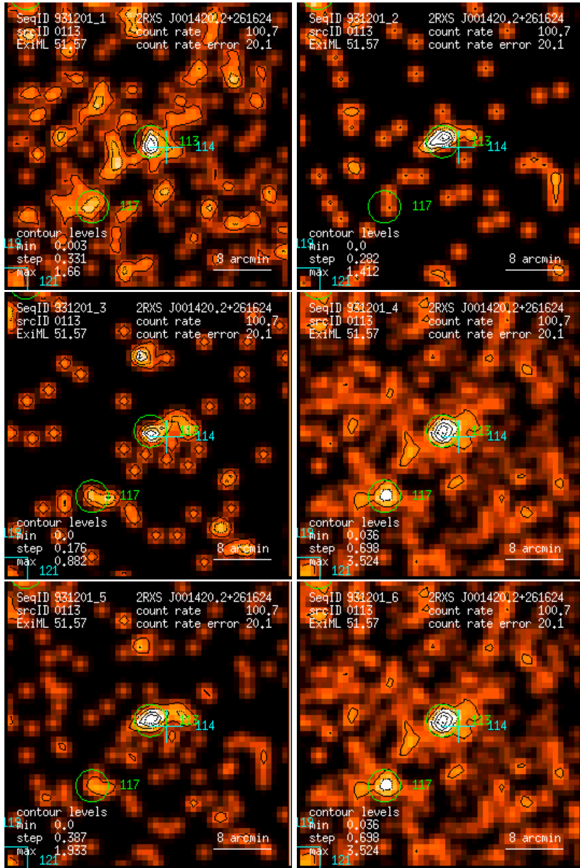
Figure 113: RASS 931201: detection 0113: band rate images, Gaussian filter: (1) PSPC channels 11 – 41, (2) 52 – 90, (3) 91 – 201, (4) 11 – 235, (5) 52 – 201, (6) 11 – 201. Broad band rates in counts/ks. Band rate contour levels in counts/ks/arcmin 2 .
