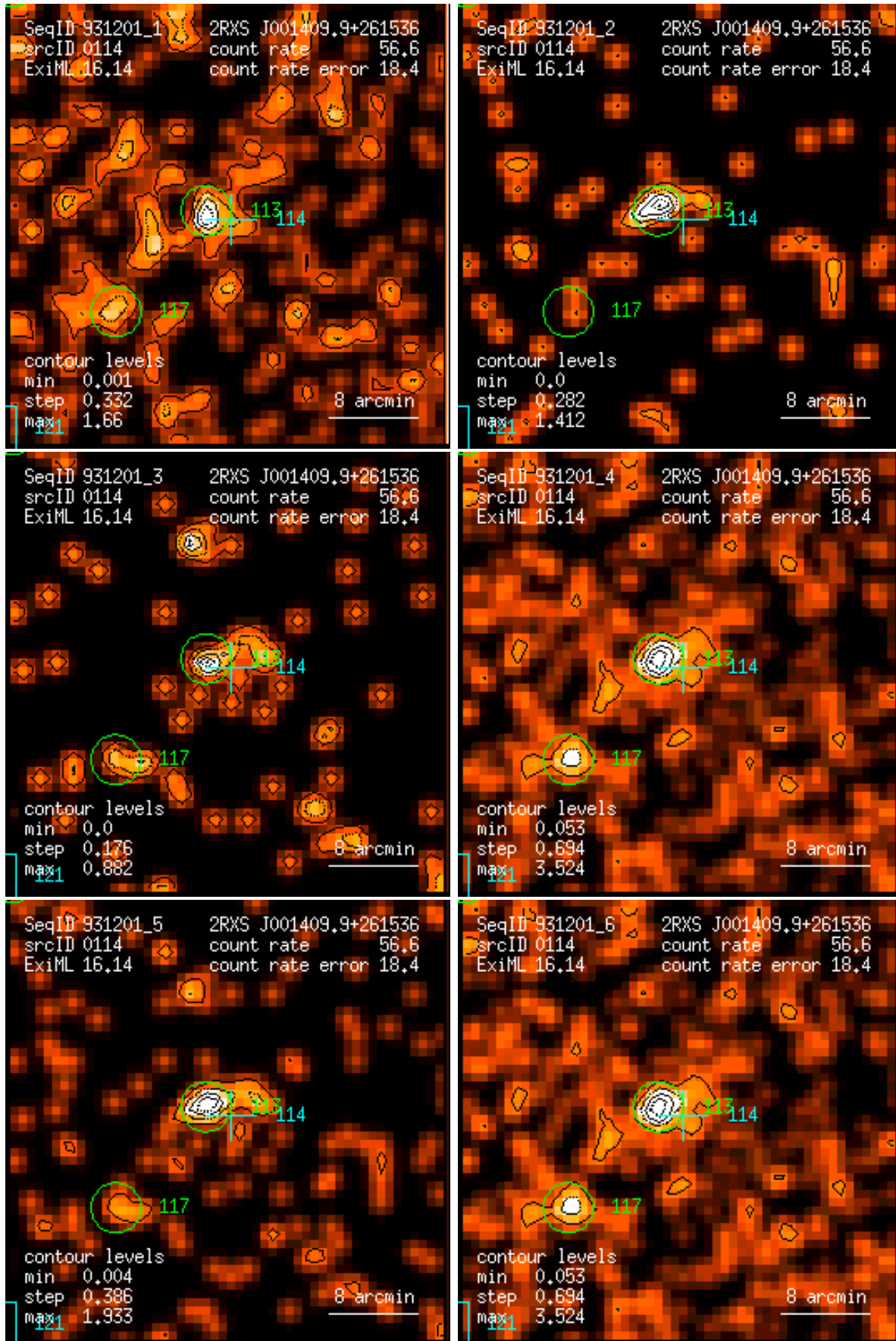
Figure 114: RASS 931201: detection 0114: band rate images, Gaussian filter: (1) PSPC channels 11 – 41, (2) 52 – 90, (3) 91 – 201, (4) 11 – 235, (5) 52 – 201, (6) 11 – 201. Broad band rates in counts/ks. Band rate contour levels in counts/ks/arcmin 2 .
