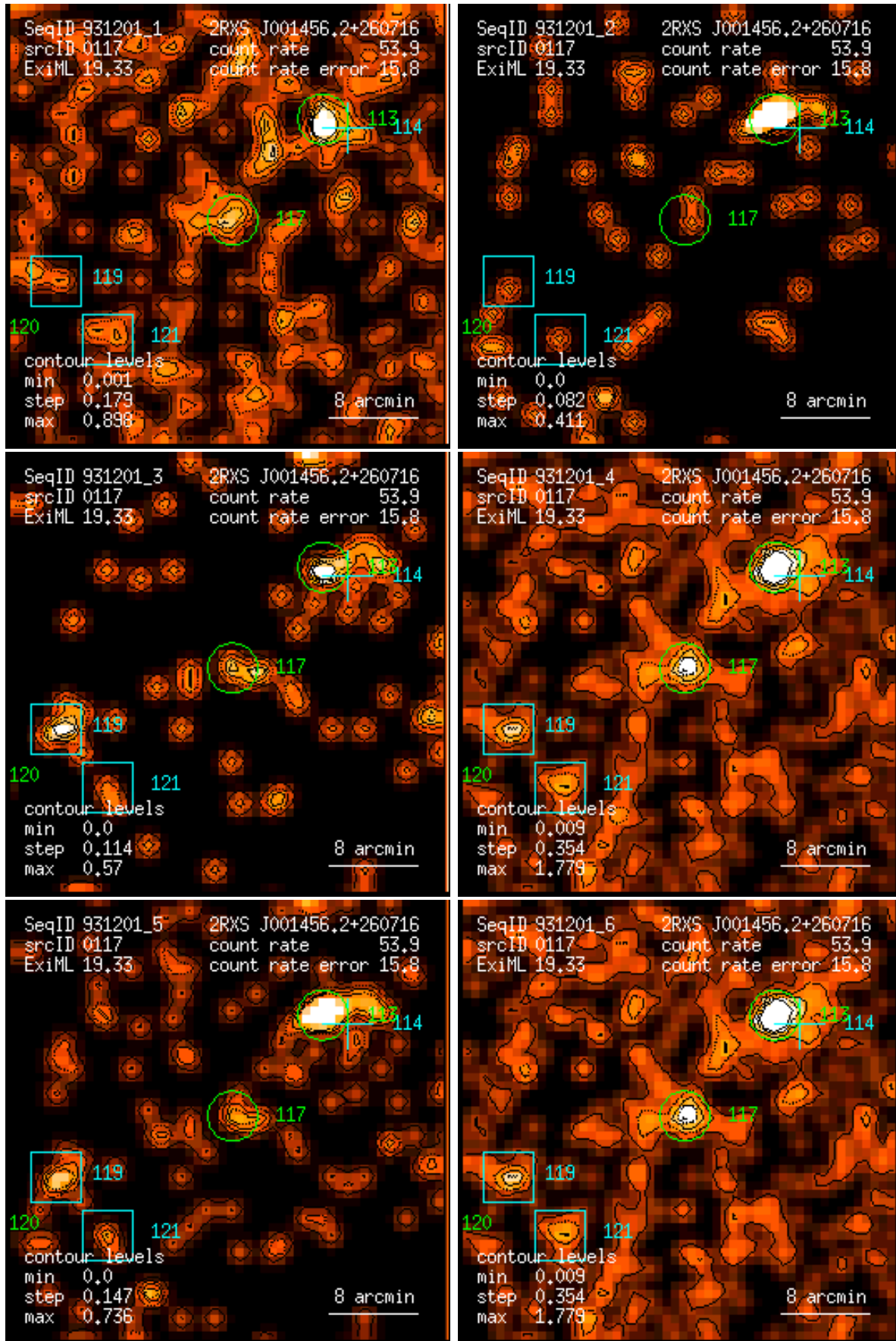
Figure 117: RASS 931201: detection 0117: band rate images, Gaussian filter: (1) PSPC channels 11 – 41, (2) 52 – 90, (3) 91 – 201, (4) 11 – 235, (5) 52 – 201, (6) 11 – 201. Broad band rates in counts/ks. Band rate contour levels in counts/ks/arcmin 2 .
