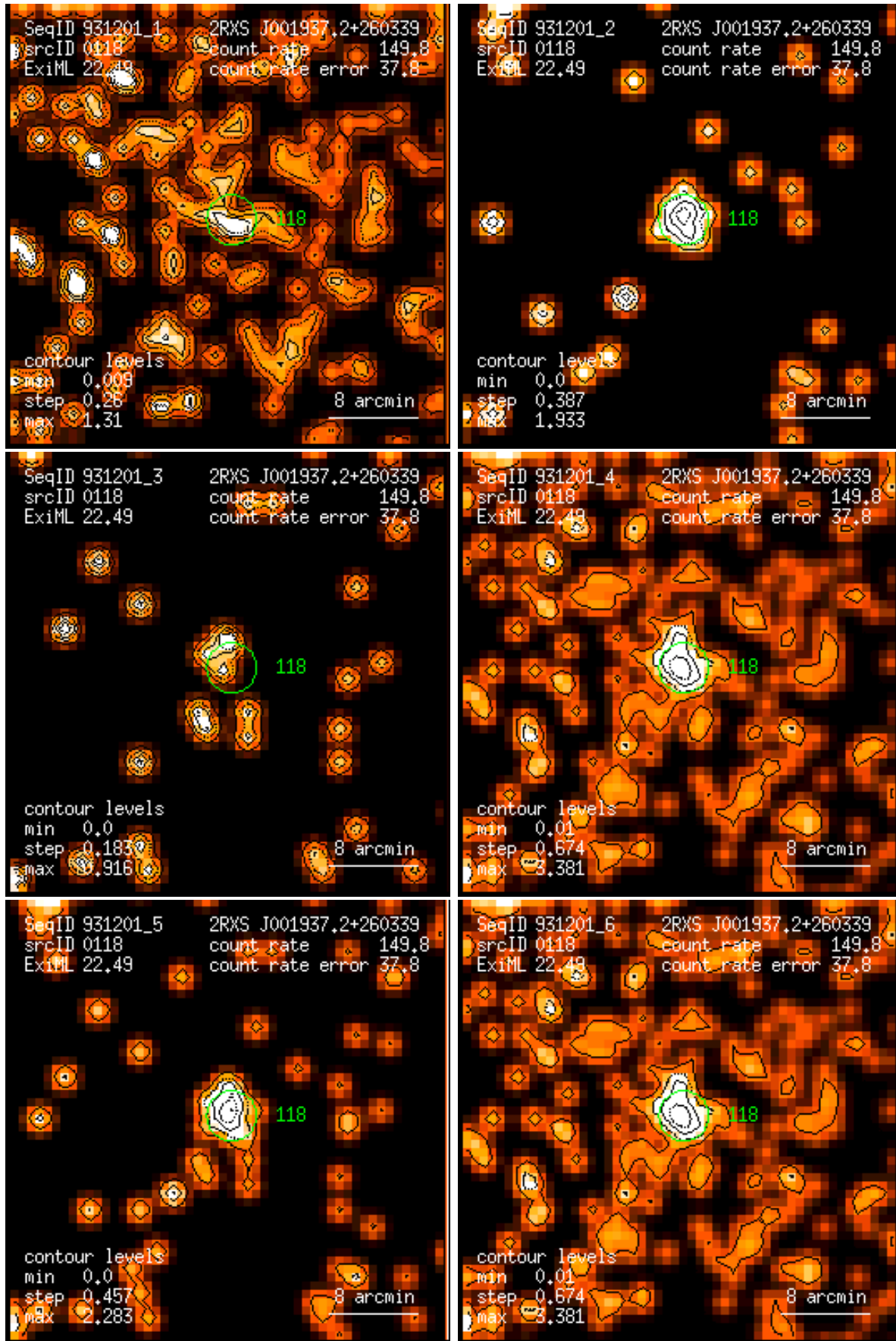
Figure 118: RASS 931201: detection 0118: band rate images, Gaussian filter: (1) PSPC channels 11 – 41, (2) 52 – 90, (3) 91 – 201, (4) 11 – 235, (5) 52 – 201, (6) 11 – 201. Broad band rates in counts/ks. Band rate contour levels in counts/ks/arcmin 2 .
