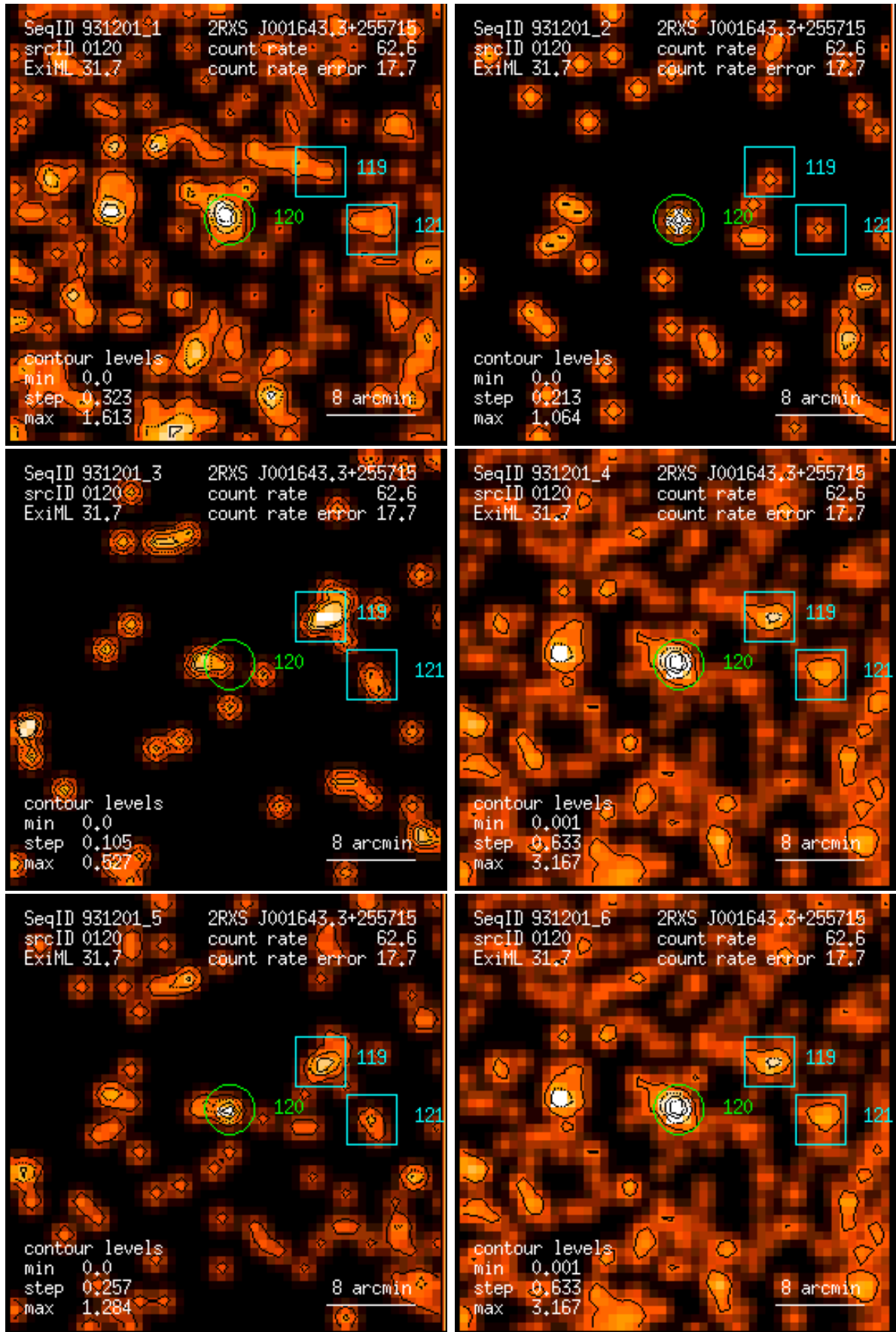
Figure 120: RASS 931201: detection 0120: band rate images, Gaussian filter: (1) PSPC channels 11 – 41, (2) 52 – 90, (3) 91 – 201, (4) 11 – 235, (5) 52 – 201, (6) 11 – 201. Broad band rates in counts/ks. Band rate contour levels in counts/ks/arcmin 2 .
